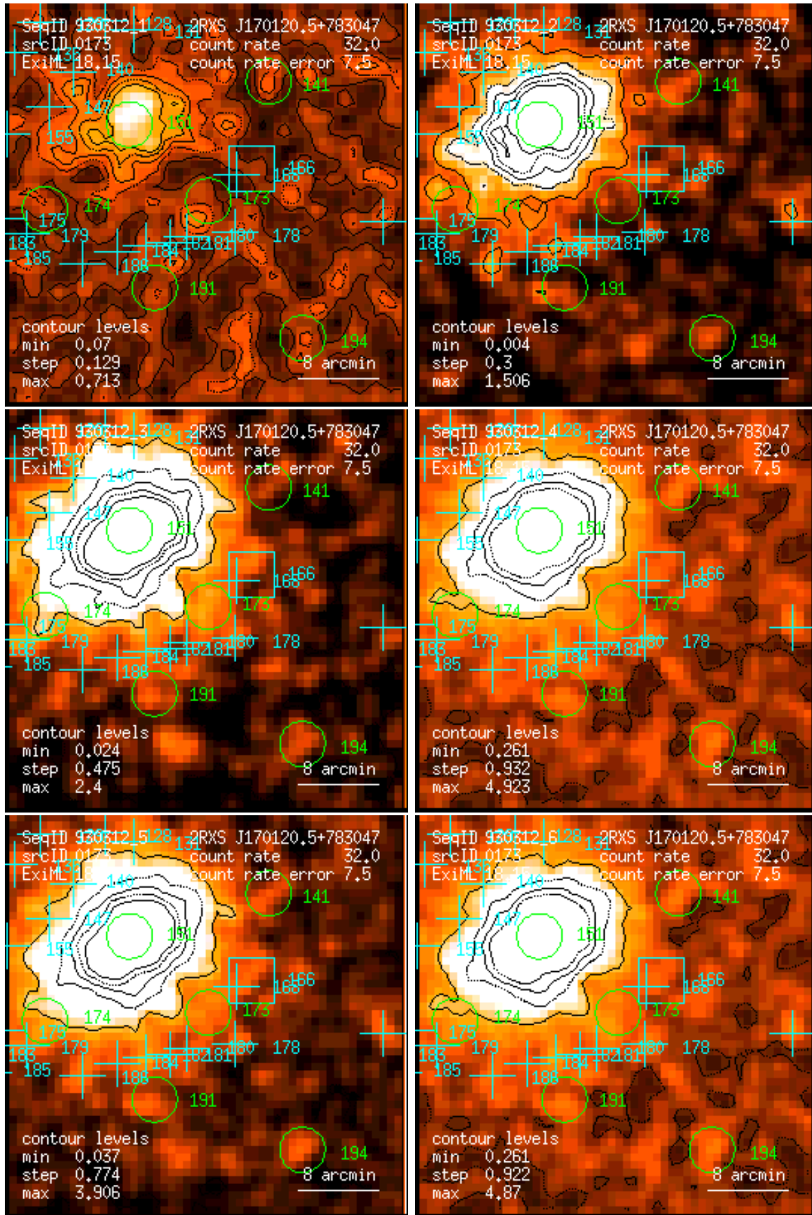
Figure 173: RASS 930312: detection 0173: band rate images, Gaussian filter: (1) PSPC channels 11 – 41, (2) 52 – 90, (3) 91 – 201, (4) 11 – 235, (5) 52 – 201, (6) 11 – 201. Broad band rates in counts/ks. Band rate contour levels in counts/ks/arcmin 2 .
