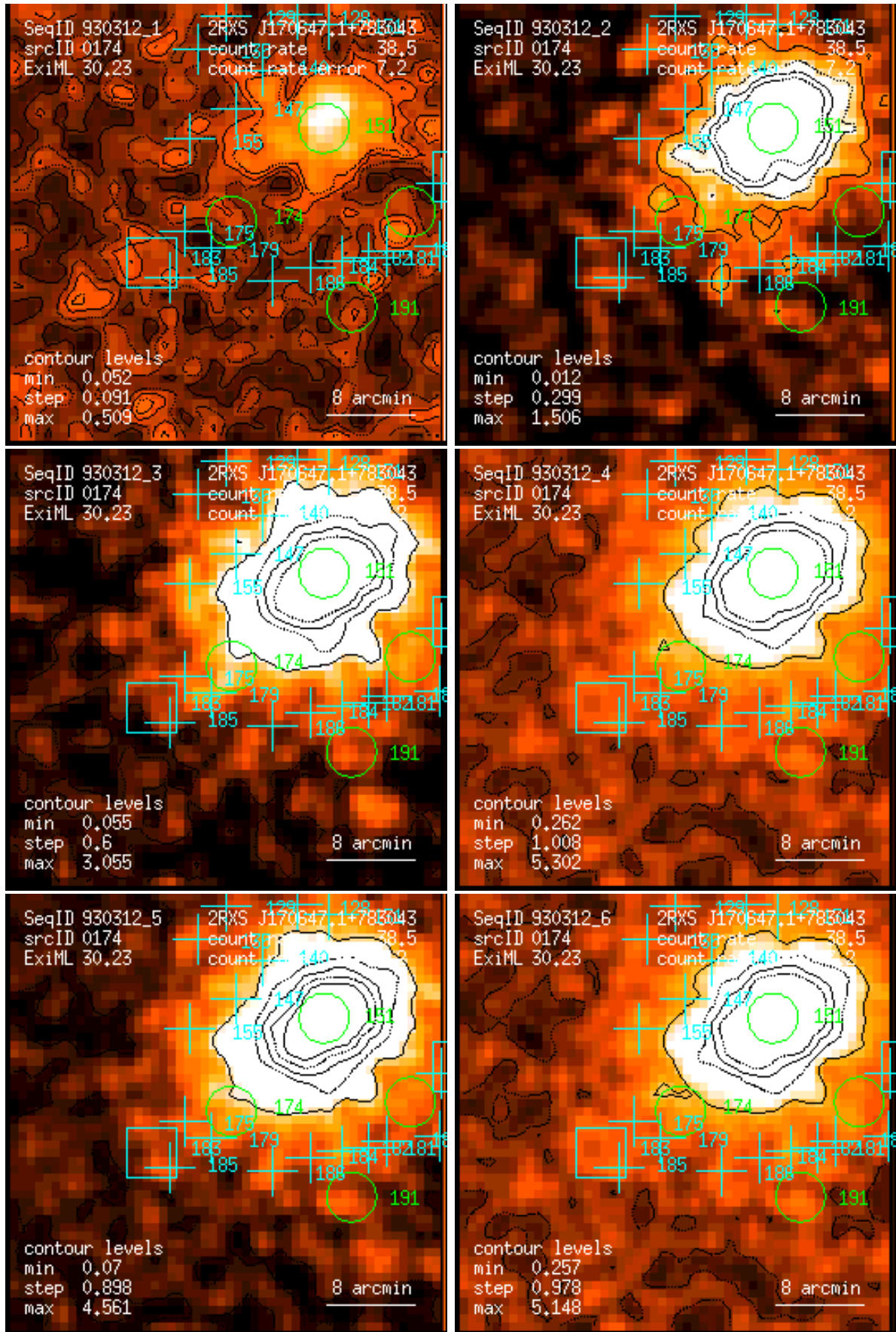
Figure 174: RASS 930312: detection 0174: band rate images, Gaussian filter: (1) PSPC channels 11 – 41, (2) 52 – 90, (3) 91 – 201, (4) 11 – 235, (5) 52 – 201, (6) 11 – 201. Broad band rates in counts/ks. Band rate contour levels in counts/ks/arcmin 2 .
