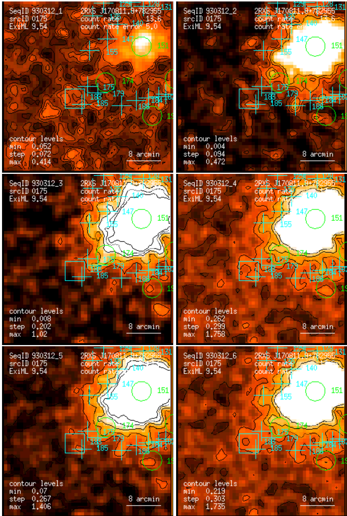
Figure 175: RASS 930312: detection 0175: band rate images, Gaussian filter: (1) PSPC channels 11 – 41, (2) 52 – 90, (3) 91 – 201, (4) 11 – 235, (5) 52 – 201, (6) 11 – 201. Broad band rates in counts/ks. Band rate contour levels in counts/ks/arcmin 2 .
