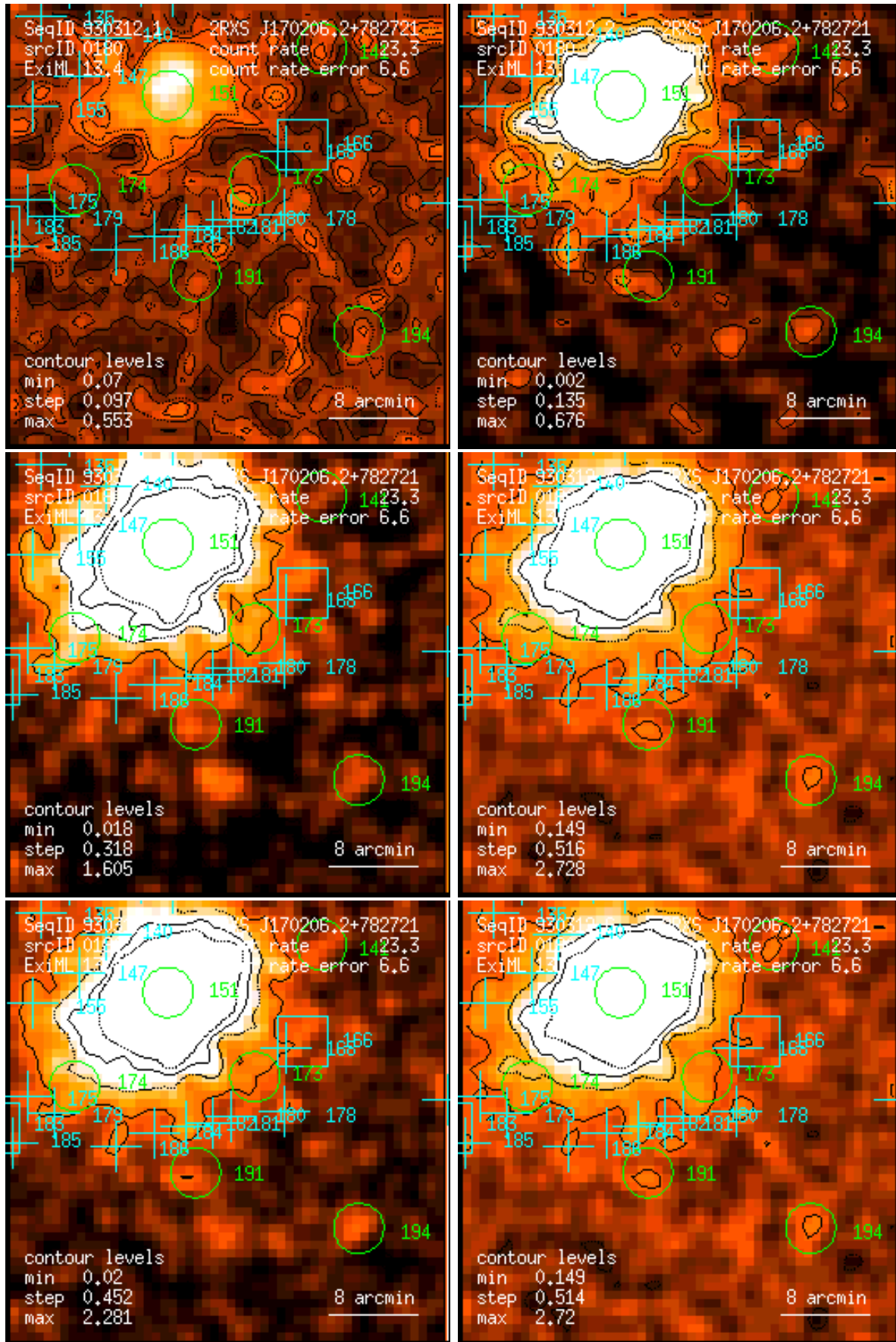
Figure 180: RASS 930312: detection 0180: band rate images, Gaussian filter: (1) PSPC channels 11 – 41, (2) 52 – 90, (3) 91 – 201, (4) 11 – 235, (5) 52 – 201, (6) 11 – 201. Broad band rates in counts/ks. Band rate contour levels in counts/ks/arcmin 2 .
