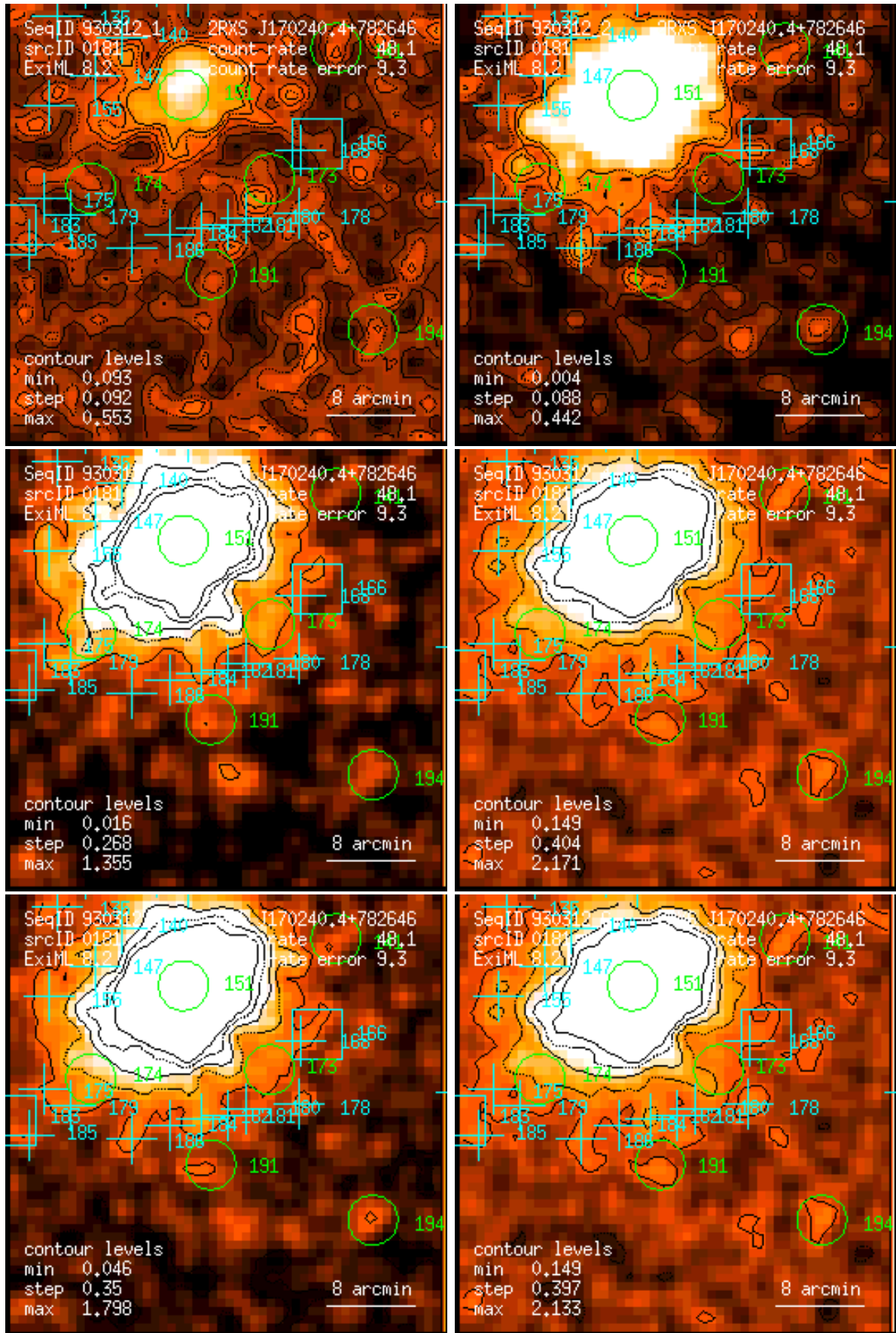
Figure 181: RASS 930312: detection 0181: band rate images, Gaussian filter: (1) PSPC channels 11 – 41, (2) 52 – 90, (3) 91 – 201, (4) 11 – 235, (5) 52 – 201, (6) 11 – 201. Broad band rates in counts/ks. Band rate contour levels in counts/ks/arcmin 2 .
