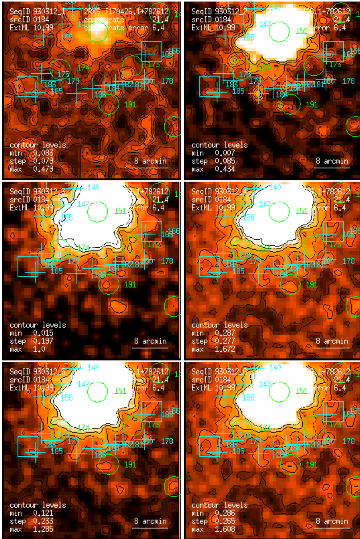
Figure 184: RASS 930312: detection 0184: band rate images, Gaussian filter: (1) PSPC channels 11 – 41, (2) 52 – 90, (3) 91 – 201, (4) 11 – 235, (5) 52 – 201, (6) 11 – 201. Broad band rates in counts/ks. Band rate contour levels in counts/ks/arcmin 2 .
