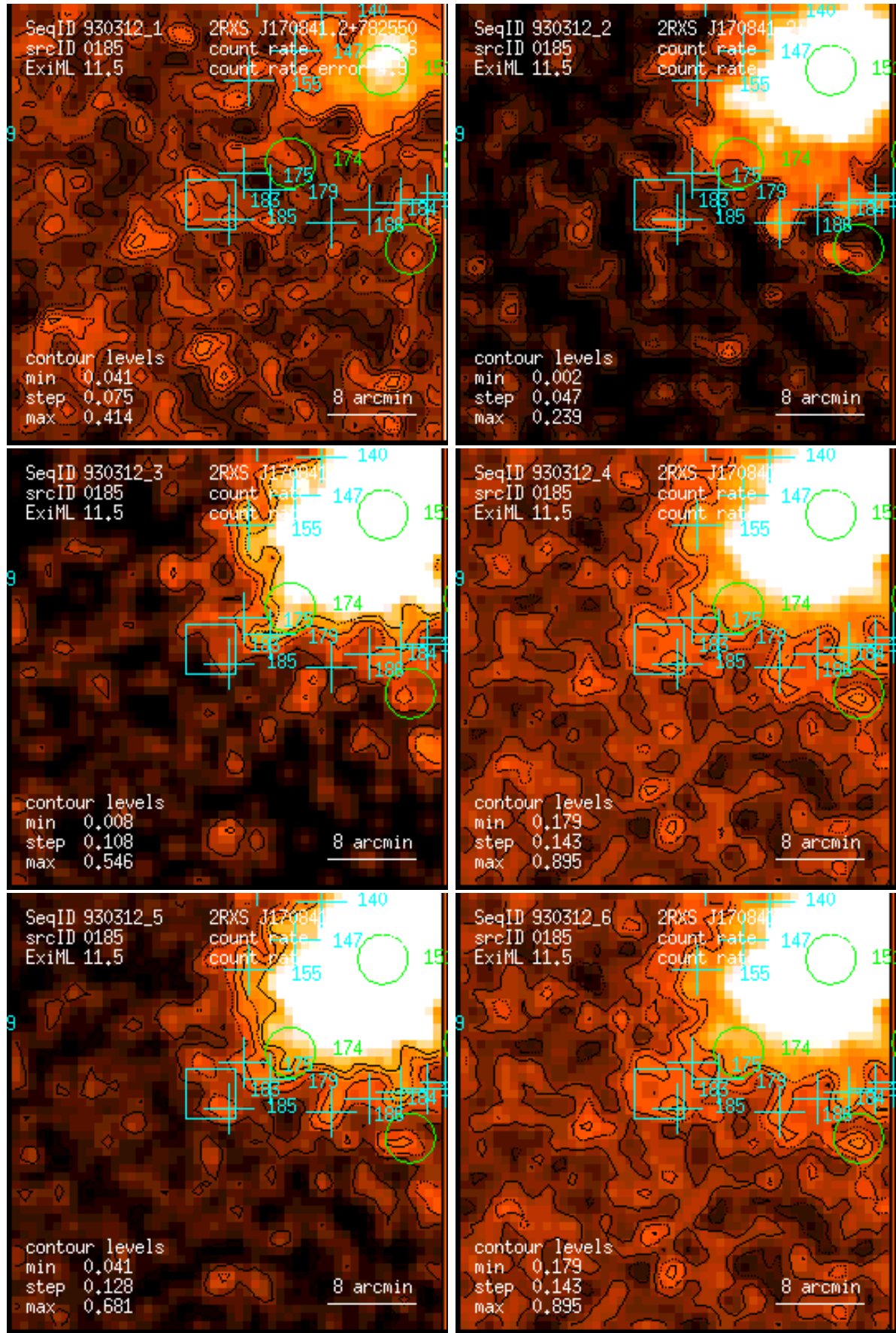
Figure 185: RASS 930312: detection 0185: band rate images, Gaussian filter: (1) PSPC channels 11 – 41, (2) 52 – 90, (3) 91 – 201, (4) 11 – 235, (5) 52 – 201, (6) 11 – 201. Broad band rates in counts/ks. Band rate contour levels in counts/ks/arcmin 2 .
