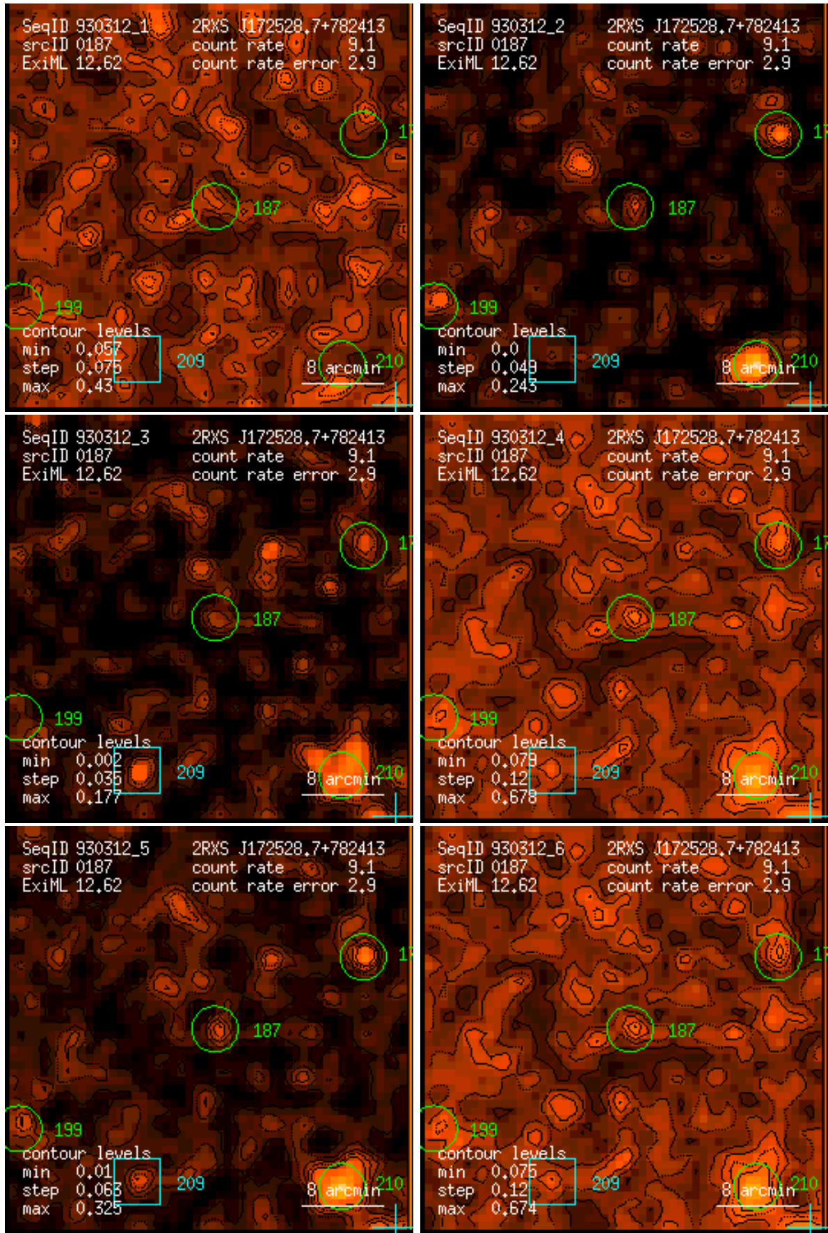
Figure 187: RASS 930312: detection 0187: band rate images, Gaussian filter: (1) PSPC channels 11 – 41, (2) 52 – 90, (3) 91 – 201, (4) 11 – 235, (5) 52 – 201, (6) 11 – 201. Broad band rates in counts/ks. Band rate contour levels in counts/ks/arcmin 2 .
