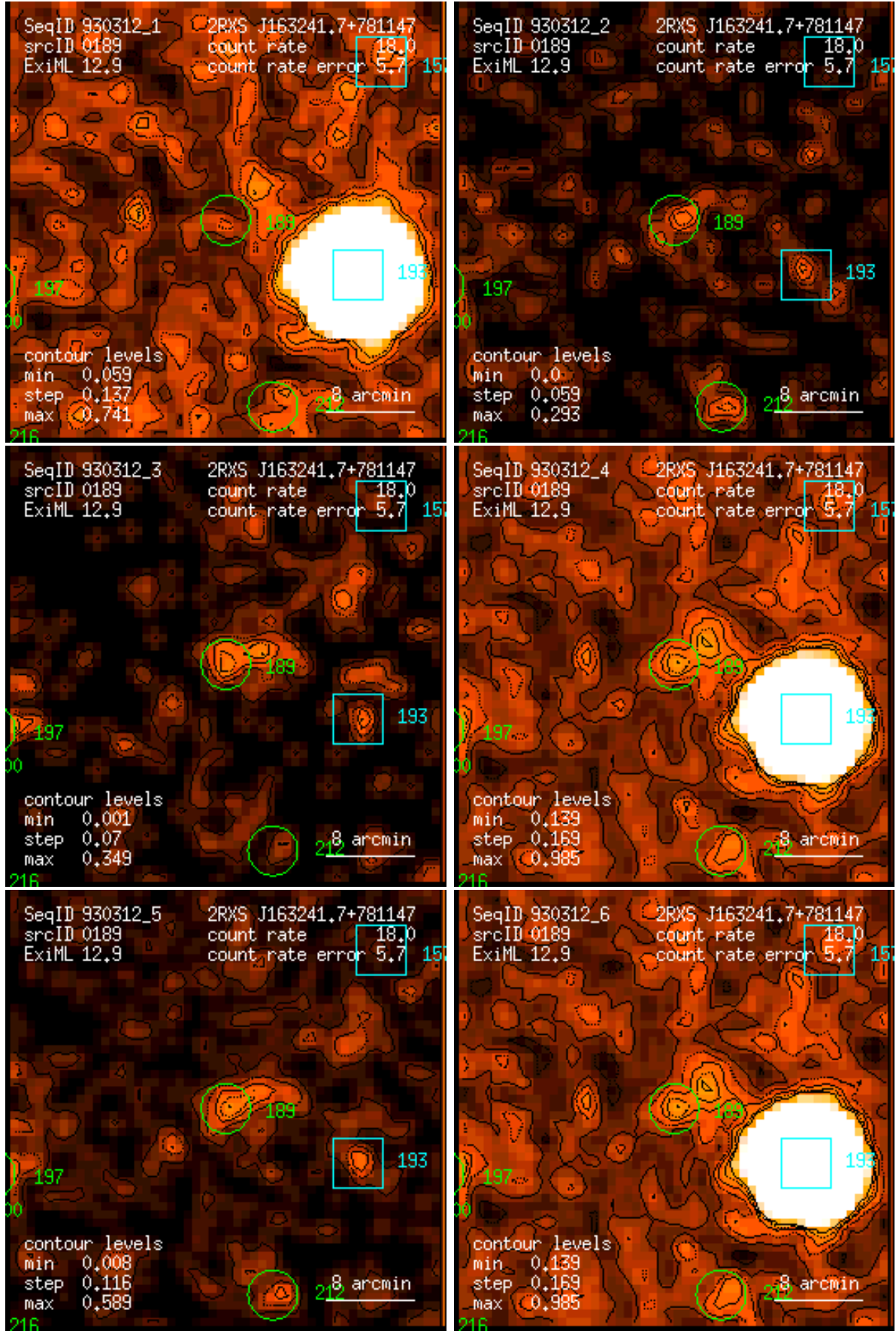
Figure 189: RASS 930312: detection 0189: band rate images, Gaussian filter: (1) PSPC channels 11 – 41, (2) 52 – 90, (3) 91 – 201, (4) 11 – 235, (5) 52 – 201, (6) 11 – 201. Broad band rates in counts/ks. Band rate contour levels in counts/ks/arcmin 2 .
