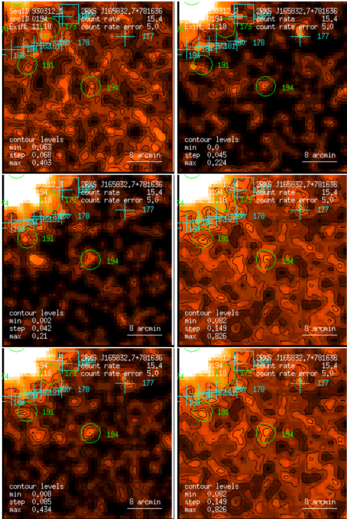
Figure 194: RASS 930312: detection 0194: band rate images, Gaussian filter: (1) PSPC channels 11 – 41, (2) 52 – 90, (3) 91 – 201, (4) 11 – 235, (5) 52 – 201, (6) 11 – 201. Broad band rates in counts/ks. Band rate contour levels in counts/ks/arcmin 2 .
