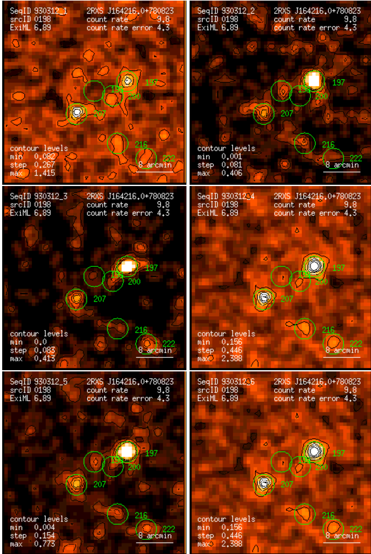
Figure 198: RASS 930312: detection 0198: band rate images, Gaussian filter: (1) PSPC channels 11 – 41, (2) 52 – 90, (3) 91 – 201, (4) 11 – 235, (5) 52 – 201, (6) 11 – 201. Broad band rates in counts/ks. Band rate contour levels in counts/ks/arcmin 2 .
