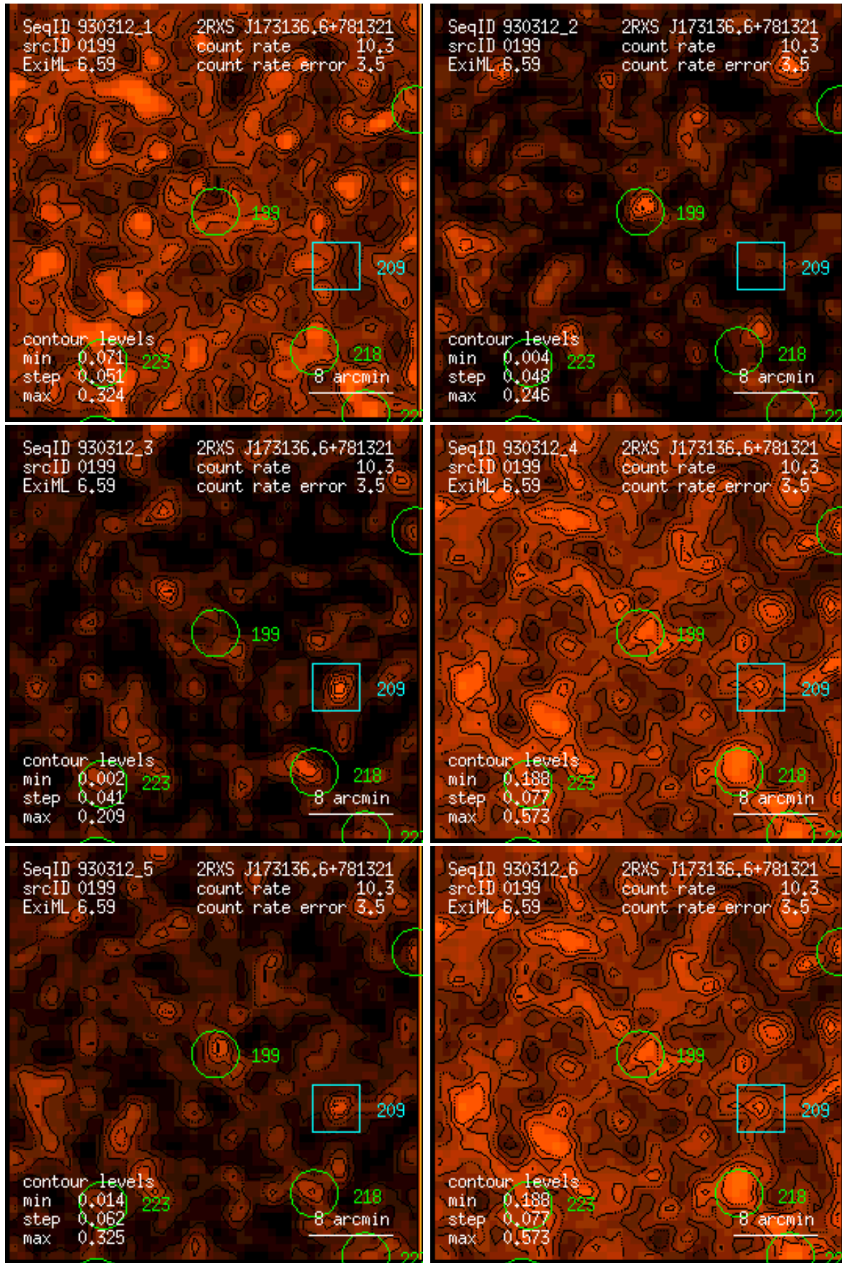
Figure 199: RASS 930312: detection 0199: band rate images, Gaussian filter: (1) PSPC channels 11 – 41, (2) 52 – 90, (3) 91 – 201, (4) 11 – 235, (5) 52 – 201, (6) 11 – 201. Broad band rates in counts/ks. Band rate contour levels in counts/ks/arcmin 2 .
