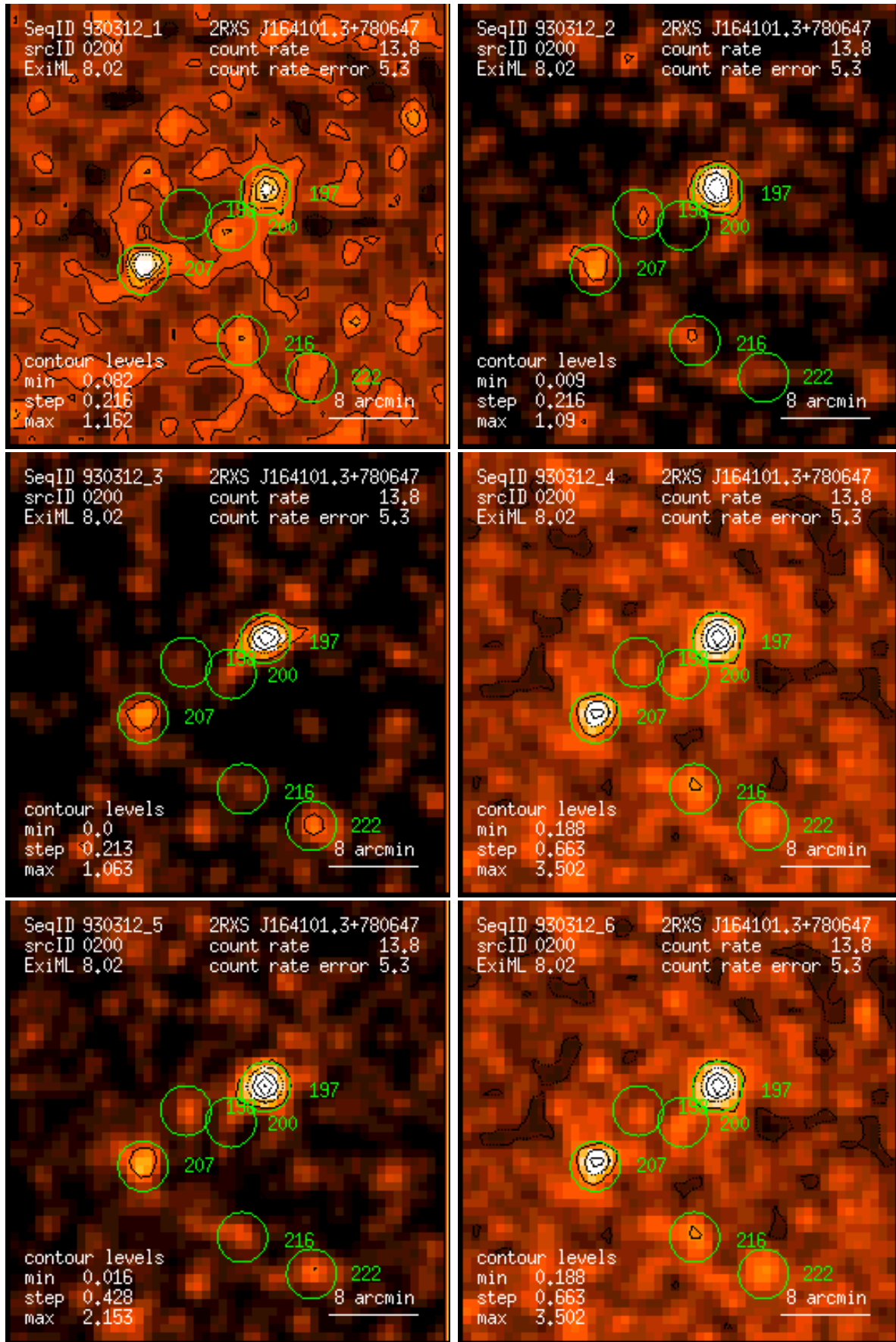
Figure 200: RASS 930312: detection 0200: band rate images, Gaussian filter: (1) PSPC channels 11 – 41, (2) 52 – 90, (3) 91 – 201, (4) 11 – 235, (5) 52 – 201, (6) 11 – 201. Broad band rates in counts/ks. Band rate contour levels in counts/ks/arcmin 2 .
