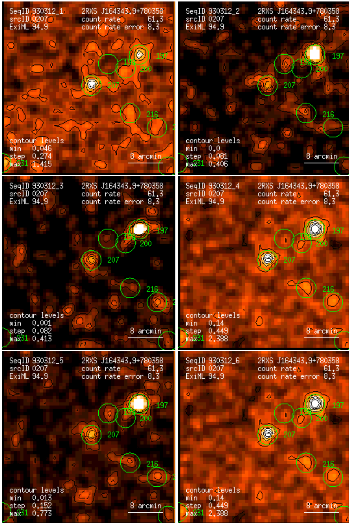
Figure 207: RASS 930312: detection 0207: band rate images, Gaussian filter: (1) PSPC channels 11 – 41, (2) 52 – 90, (3) 91 – 201, (4) 11 – 235, (5) 52 – 201, (6) 11 – 201. Broad band rates in counts/ks. Band rate contour levels in counts/ks/arcmin 2 .
