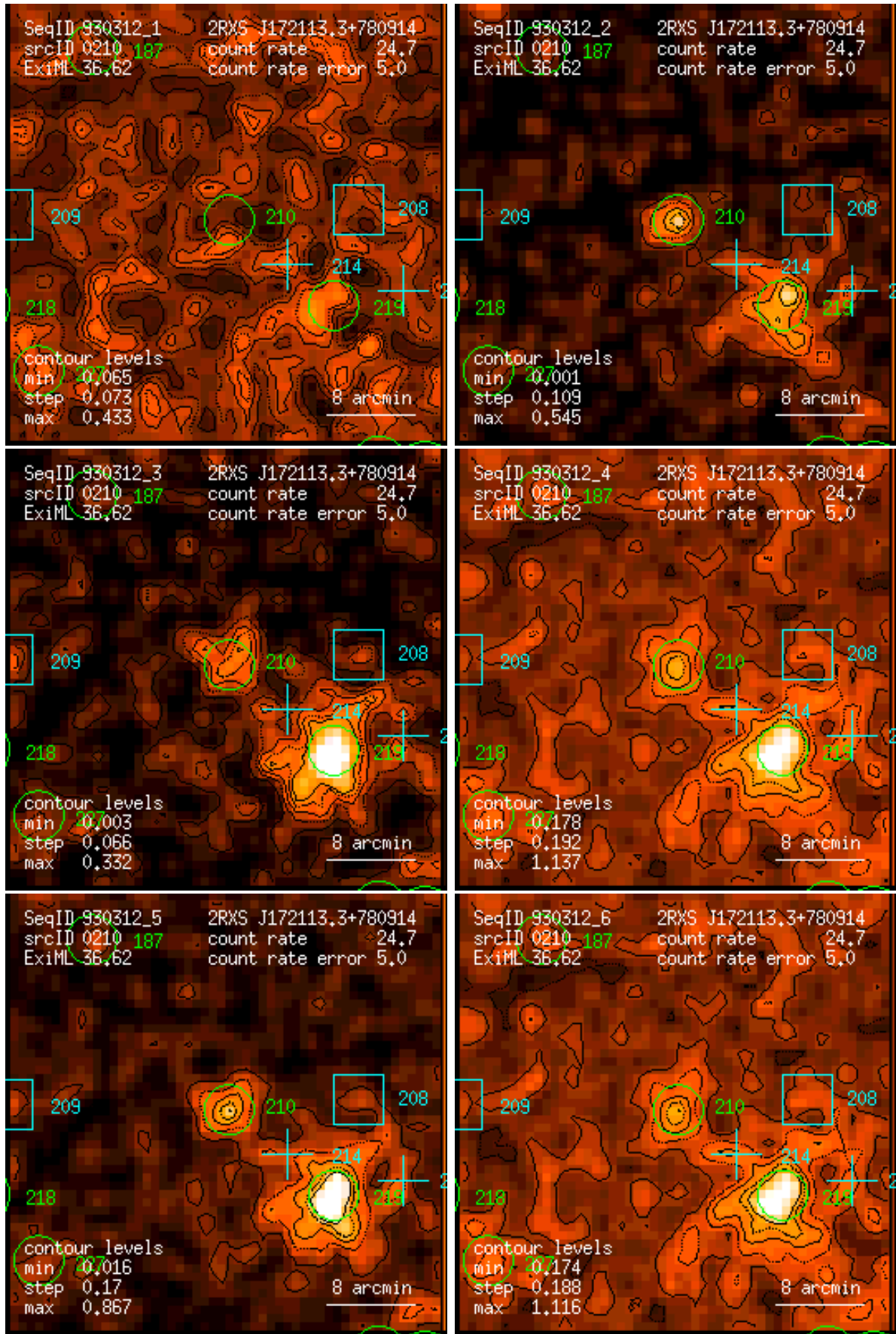
Figure 210: RASS 930312: detection 0210: band rate images, Gaussian filter: (1) PSPC channels 11 – 41, (2) 52 – 90, (3) 91 – 201, (4) 11 – 235, (5) 52 – 201, (6) 11 – 201. Broad band rates in counts/ks. Band rate contour levels in counts/ks/arcmin 2 .
