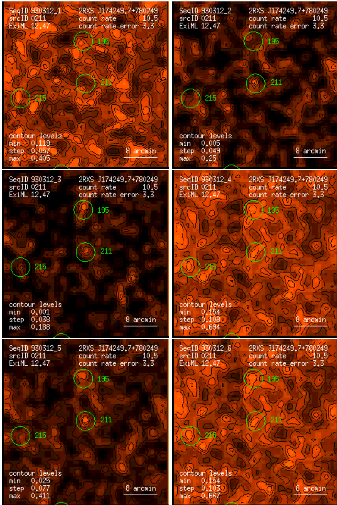
Figure 211: RASS 930312: detection 0211: band rate images, Gaussian filter: (1) PSPC channels 11 – 41, (2) 52 – 90, (3) 91 – 201, (4) 11 – 235, (5) 52 – 201, (6) 11 – 201. Broad band rates in counts/ks. Band rate contour levels in counts/ks/arcmin 2 .
