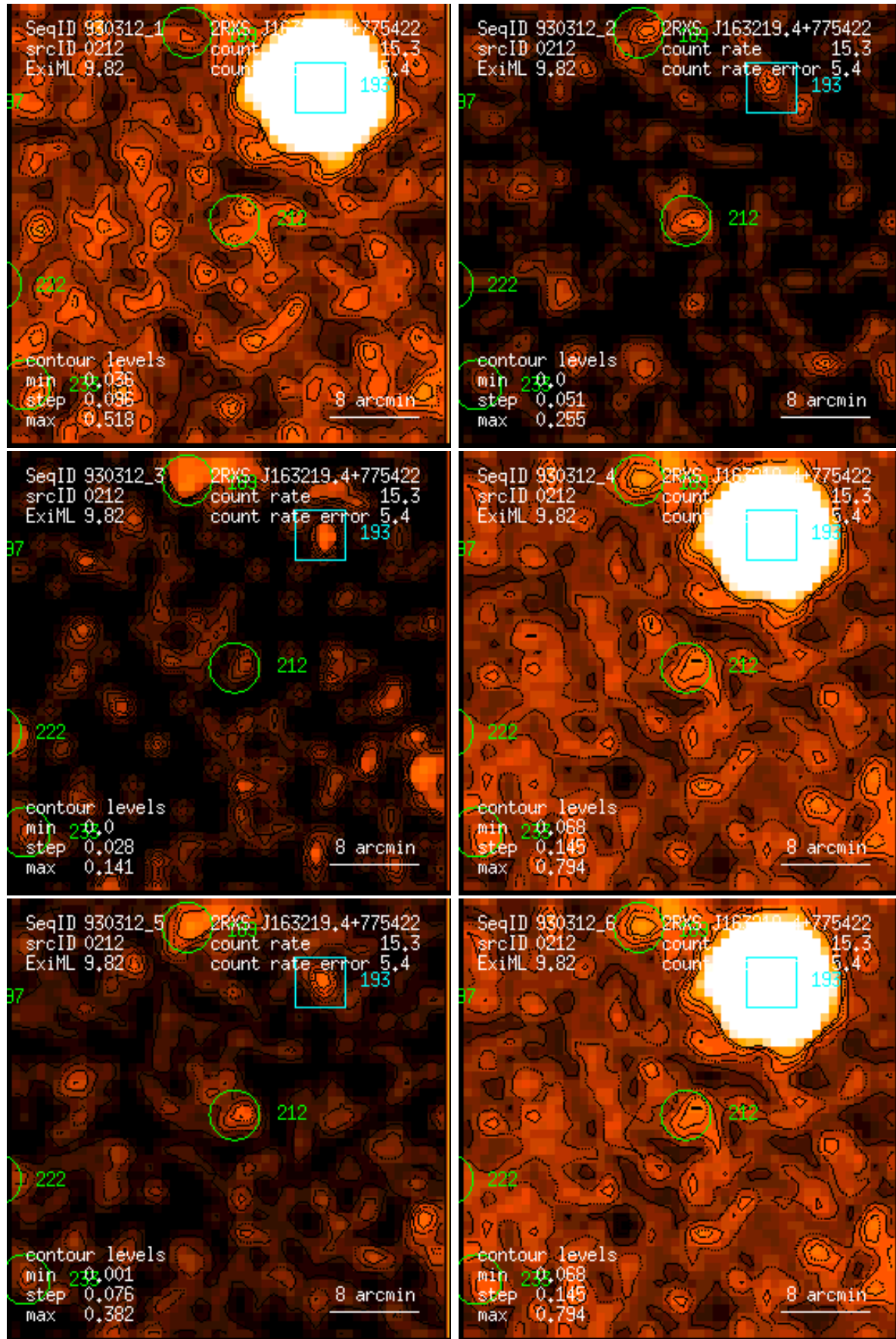
Figure 212: RASS 930312: detection 0212: band rate images, Gaussian filter: (1) PSPC channels 11 – 41, (2) 52 – 90, (3) 91 – 201, (4) 11 – 235, (5) 52 – 201, (6) 11 – 201. Broad band rates in counts/ks. Band rate contour levels in counts/ks/arcmin 2 .
