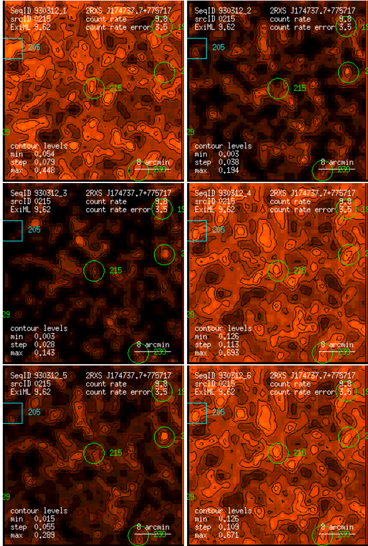
Figure 215: RASS 930312: detection 0215: band rate images, Gaussian filter: (1) PSPC channels 11 – 41, (2) 52 – 90, (3) 91 – 201, (4) 11 – 235, (5) 52 – 201, (6) 11 – 201. Broad band rates in counts/ks. Band rate contour levels in counts/ks/arcmin 2 .
