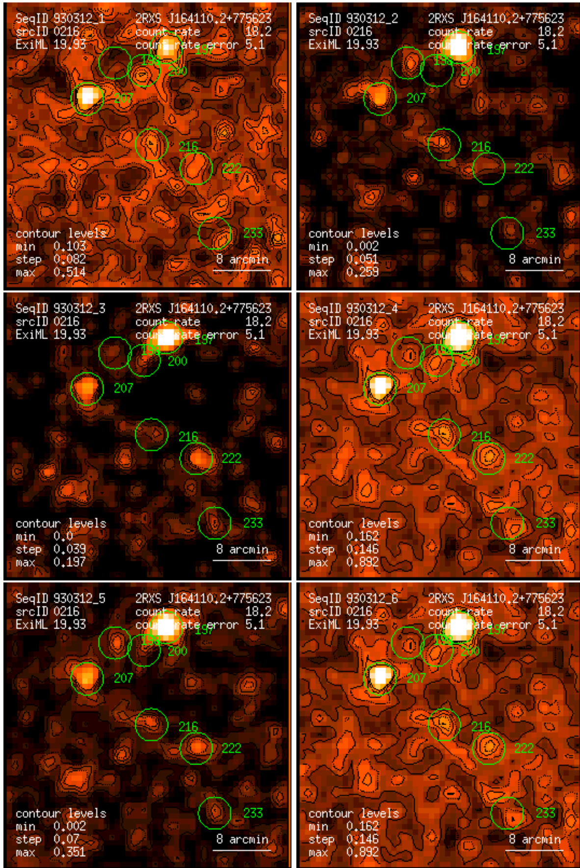
Figure 216: RASS 930312: detection 0216: band rate images, Gaussian filter: (1) PSPC channels 11 – 41, (2) 52 – 90, (3) 91 – 201, (4) 11 – 235, (5) 52 – 201, (6) 11 – 201. Broad band rates in counts/ks. Band rate contour levels in counts/ks/arcmin 2 .
