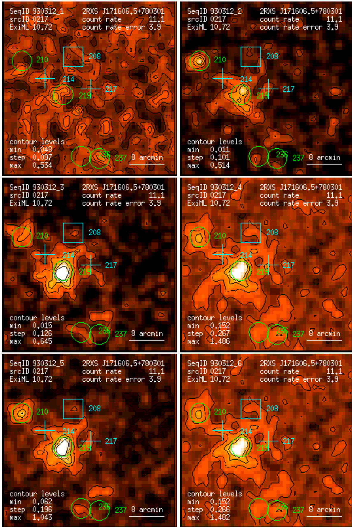
Figure 217: RASS 930312: detection 0217: band rate images, Gaussian filter: (1) PSPC channels 11 – 41, (2) 52 – 90, (3) 91 – 201, (4) 11 – 235, (5) 52 – 201, (6) 11 – 201. Broad band rates in counts/ks. Band rate contour levels in counts/ks/arcmin 2 .
