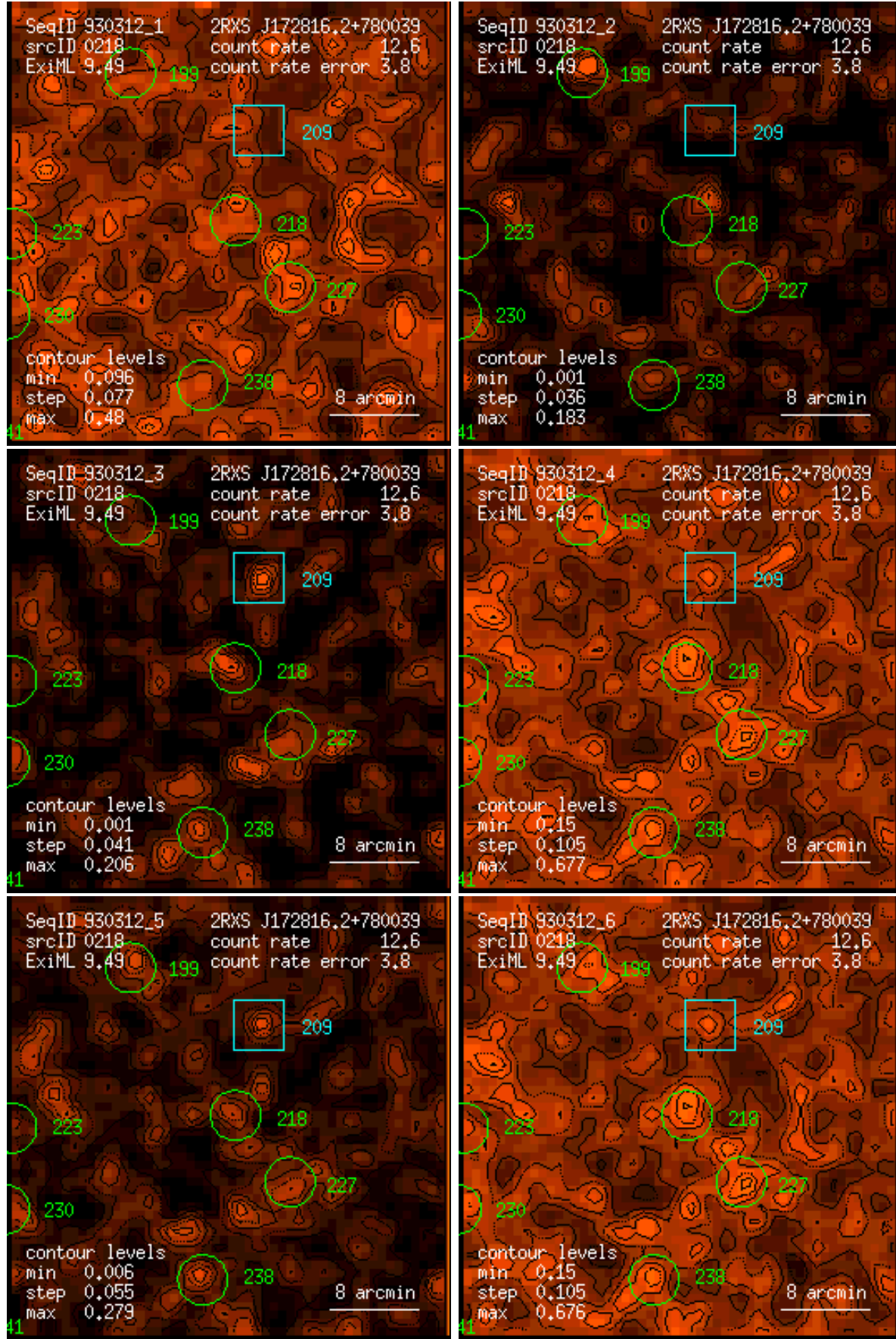
Figure 218: RASS 930312: detection 0218: band rate images, Gaussian filter: (1) PSPC channels 11 – 41, (2) 52 – 90, (3) 91 – 201, (4) 11 – 235, (5) 52 – 201, (6) 11 – 201. Broad band rates in counts/ks. Band rate contour levels in counts/ks/arcmin 2 .
