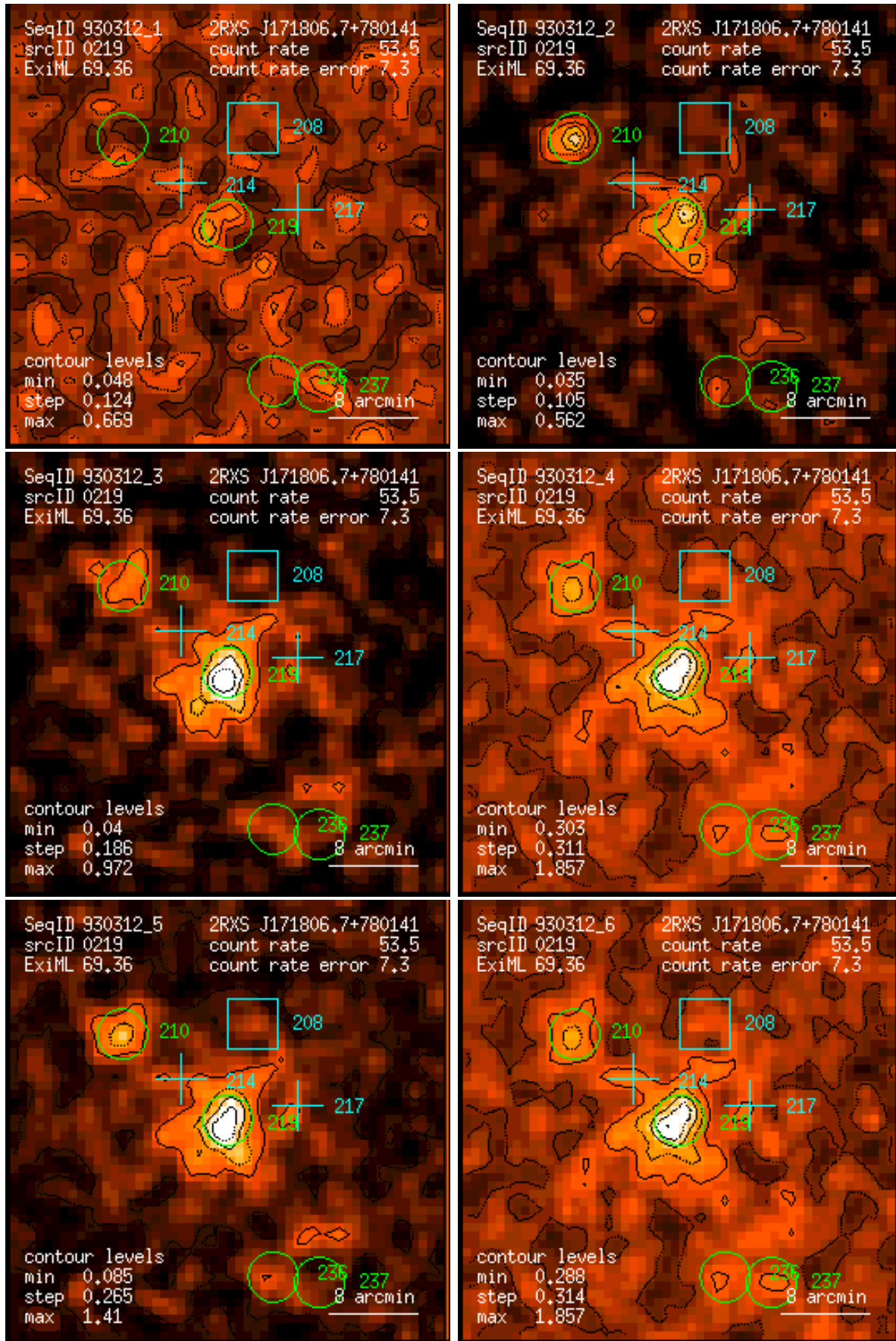
Figure 219: RASS 930312: detection 0219: band rate images, Gaussian filter: (1) PSPC channels 11 – 41, (2) 52 – 90, (3) 91 – 201, (4) 11 – 235, (5) 52 – 201, (6) 11 – 201. Broad band rates in counts/ks. Band rate contour levels in counts/ks/arcmin 2 .
