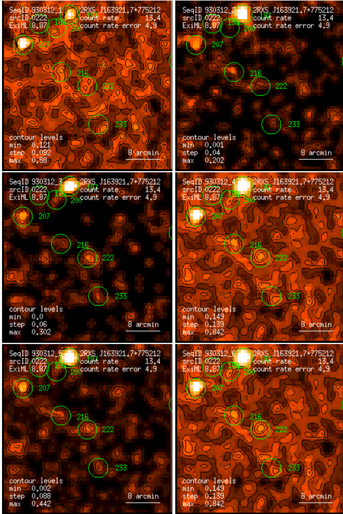
Figure 222: RASS 930312: detection 0222: band rate images, Gaussian filter: (1) PSPC channels 11 – 41, (2) 52 – 90, (3) 91 – 201, (4) 11 – 235, (5) 52 – 201, (6) 11 – 201. Broad band rates in counts/ks. Band rate contour levels in counts/ks/arcmin 2 .
