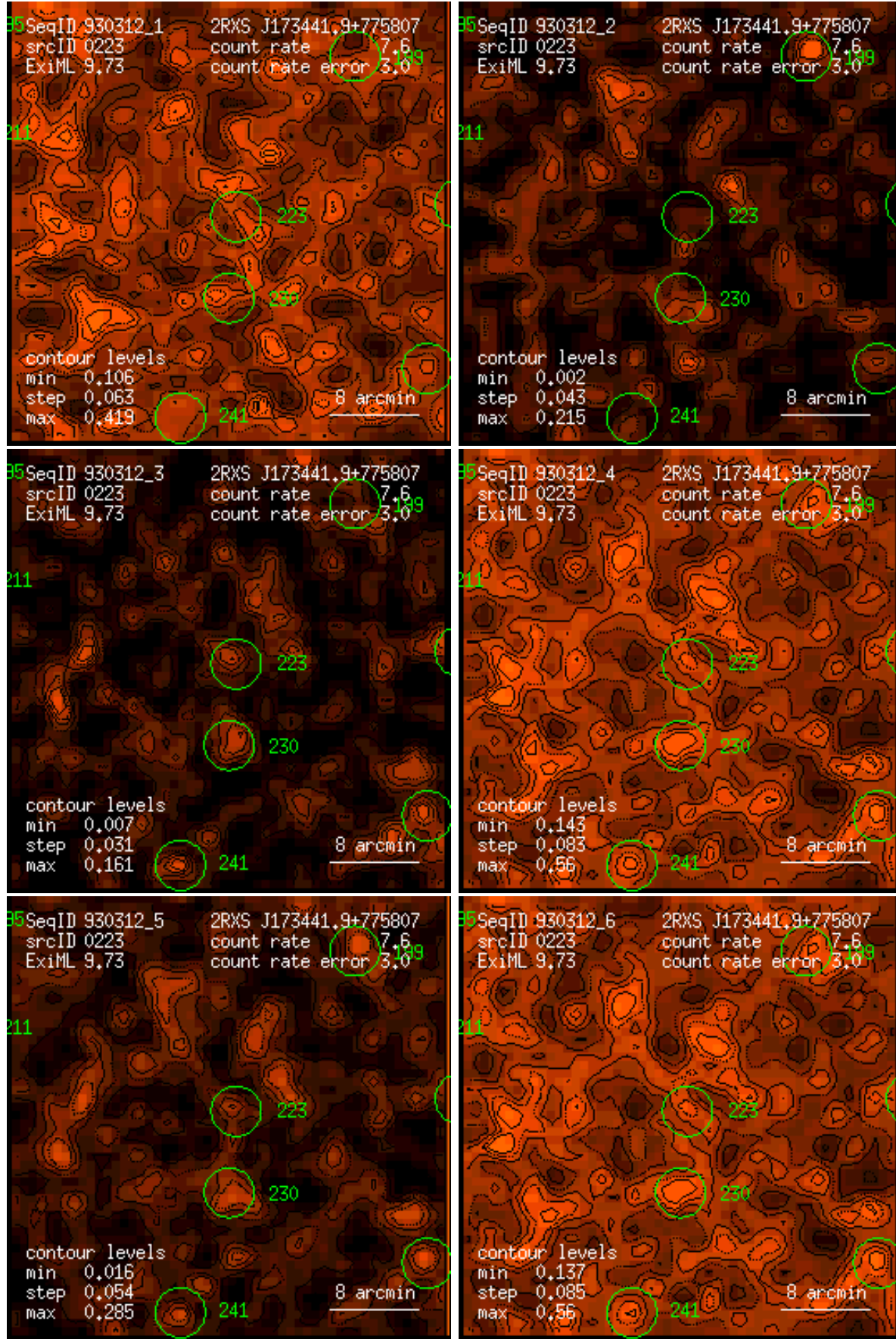
Figure 223: RASS 930312: detection 0223: band rate images, Gaussian filter: (1) PSPC channels 11 – 41, (2) 52 – 90, (3) 91 – 201, (4) 11 – 235, (5) 52 – 201, (6) 11 – 201. Broad band rates in counts/ks. Band rate contour levels in counts/ks/arcmin 2 .
