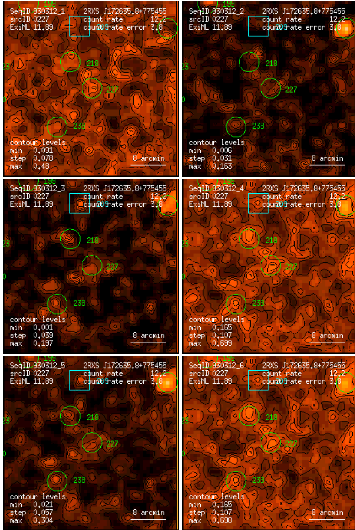
Figure 227: RASS 930312: detection 0227: band rate images, Gaussian filter: (1) PSPC channels 11 – 41, (2) 52 – 90, (3) 91 – 201, (4) 11 – 235, (5) 52 – 201, (6) 11 – 201. Broad band rates in counts/ks. Band rate contour levels in counts/ks/arcmin 2 .
