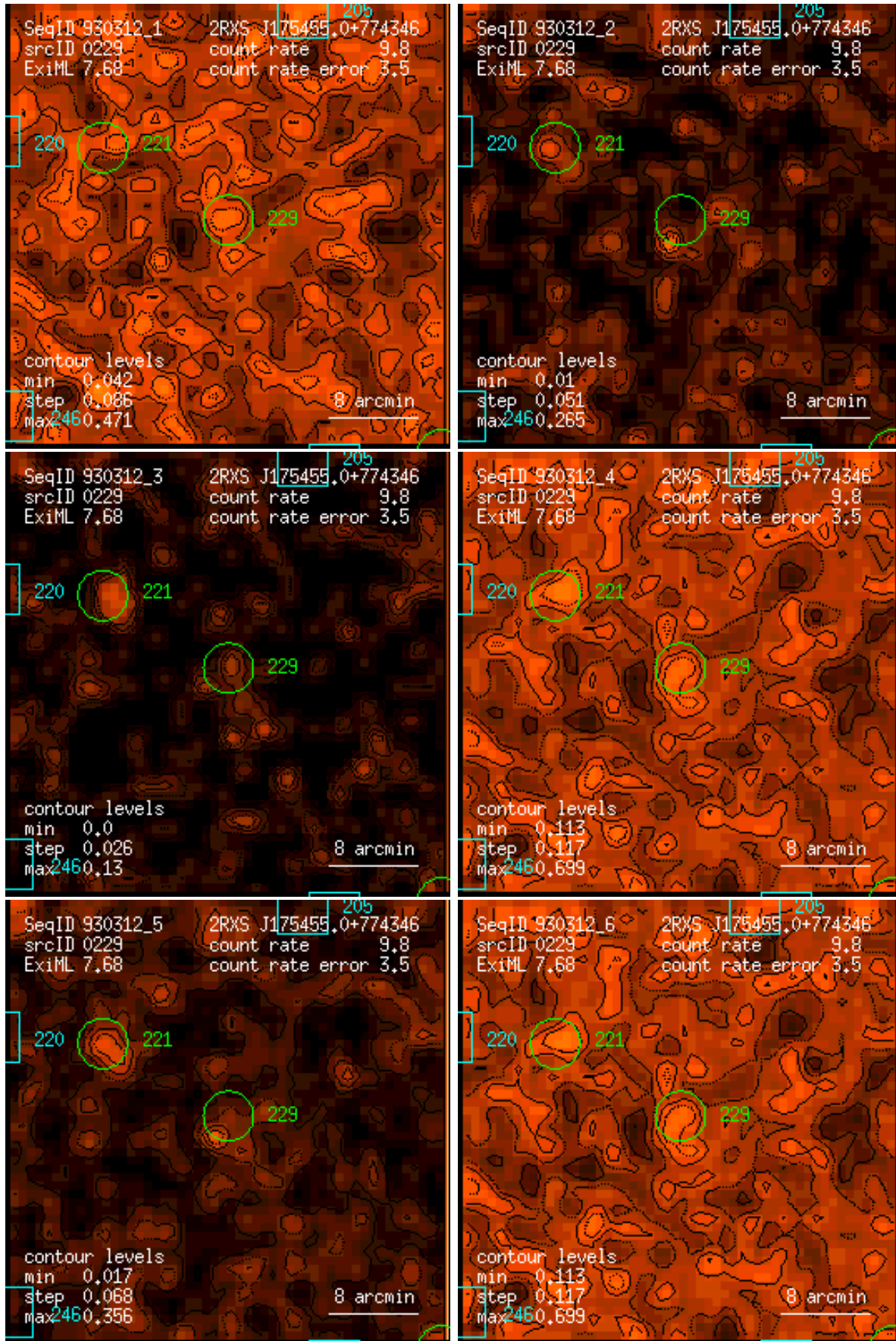
Figure 229: RASS 930312: detection 0229: band rate images, Gaussian filter: (1) PSPC channels 11 – 41, (2) 52 – 90, (3) 91 – 201, (4) 11 – 235, (5) 52 – 201, (6) 11 – 201. Broad band rates in counts/ks. Band rate contour levels in counts/ks/arcmin 2 .
