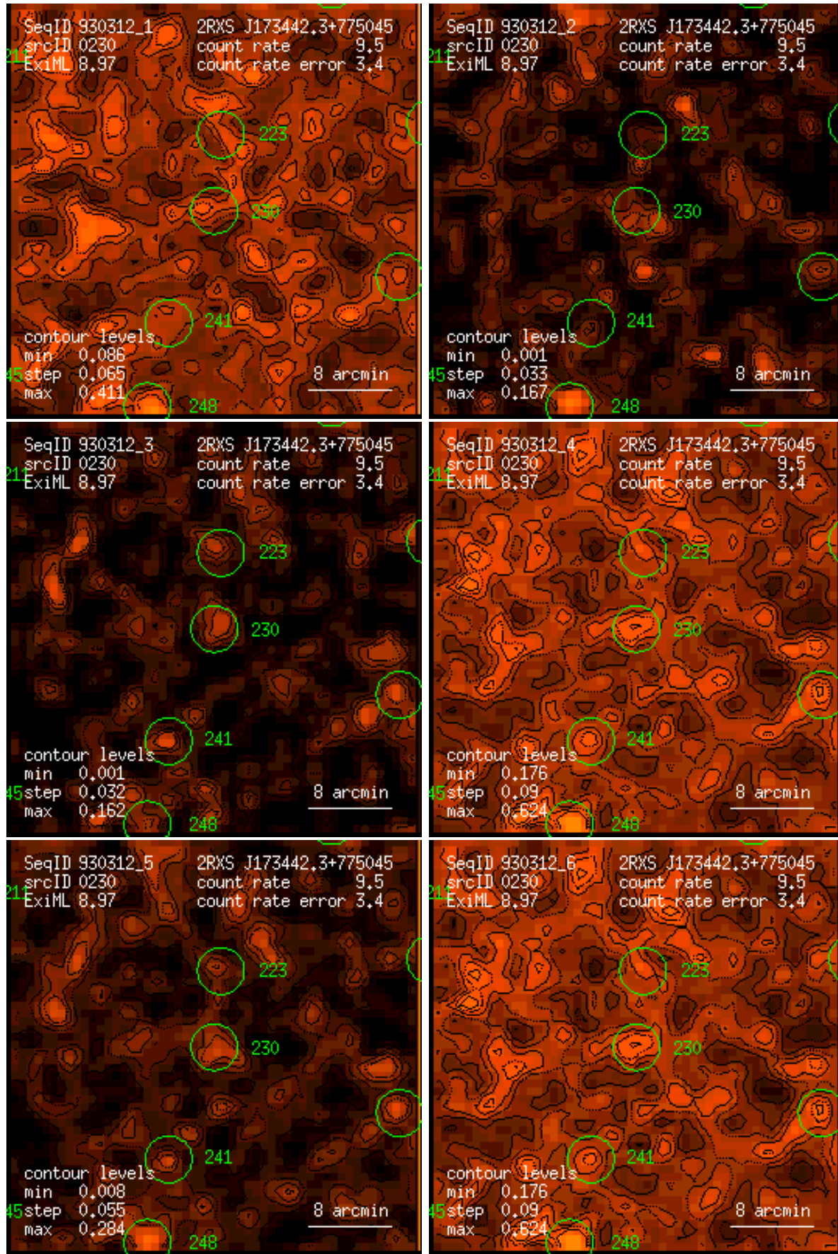
Figure 230: RASS 930312: detection 0230: band rate images, Gaussian filter: (1) PSPC channels 11 – 41, (2) 52 – 90, (3) 91 – 201, (4) 11 – 235, (5) 52 – 201, (6) 11 – 201. Broad band rates in counts/ks. Band rate contour levels in counts/ks/arcmin 2 .
