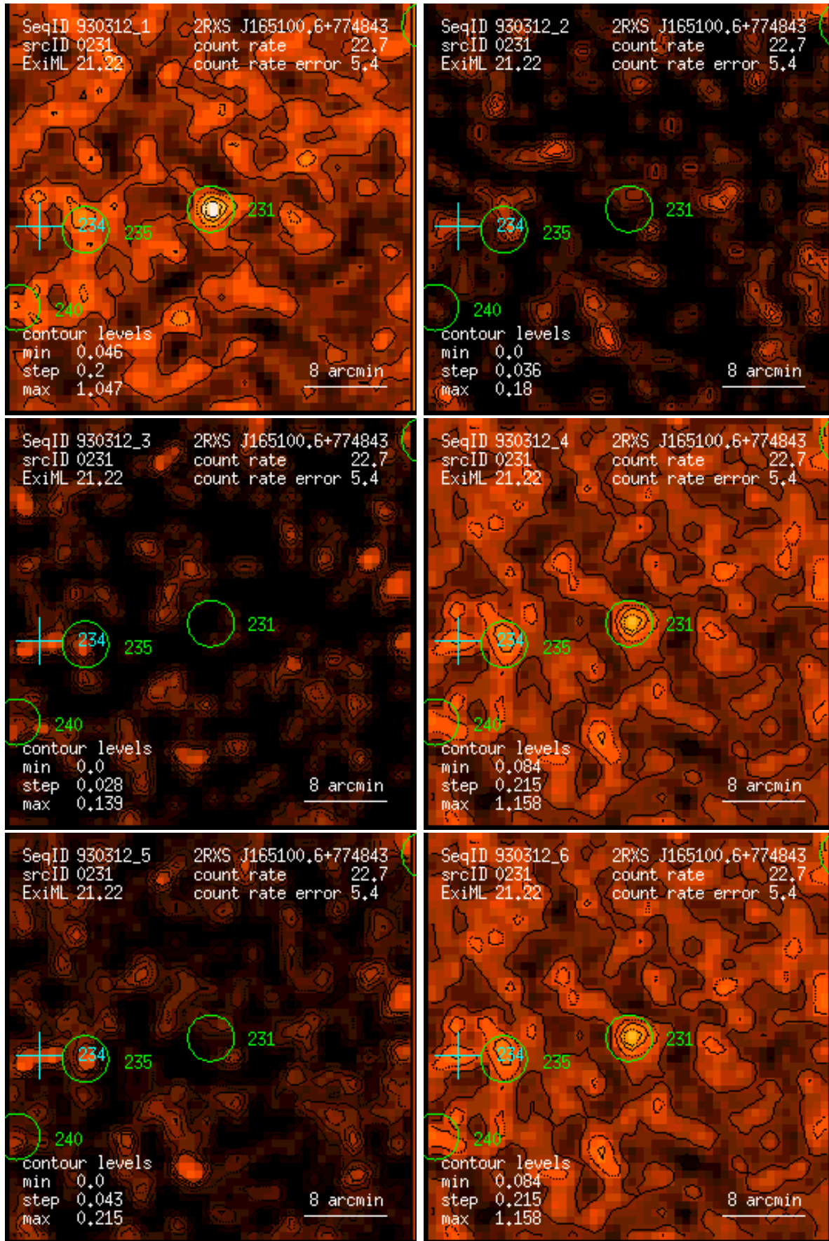
Figure 231: RASS 930312: detection 0231: band rate images, Gaussian filter: (1) PSPC channels 11 – 41, (2) 52 – 90, (3) 91 – 201, (4) 11 – 235, (5) 52 – 201, (6) 11 – 201. Broad band rates in counts/ks. Band rate contour levels in counts/ks/arcmin 2 .
