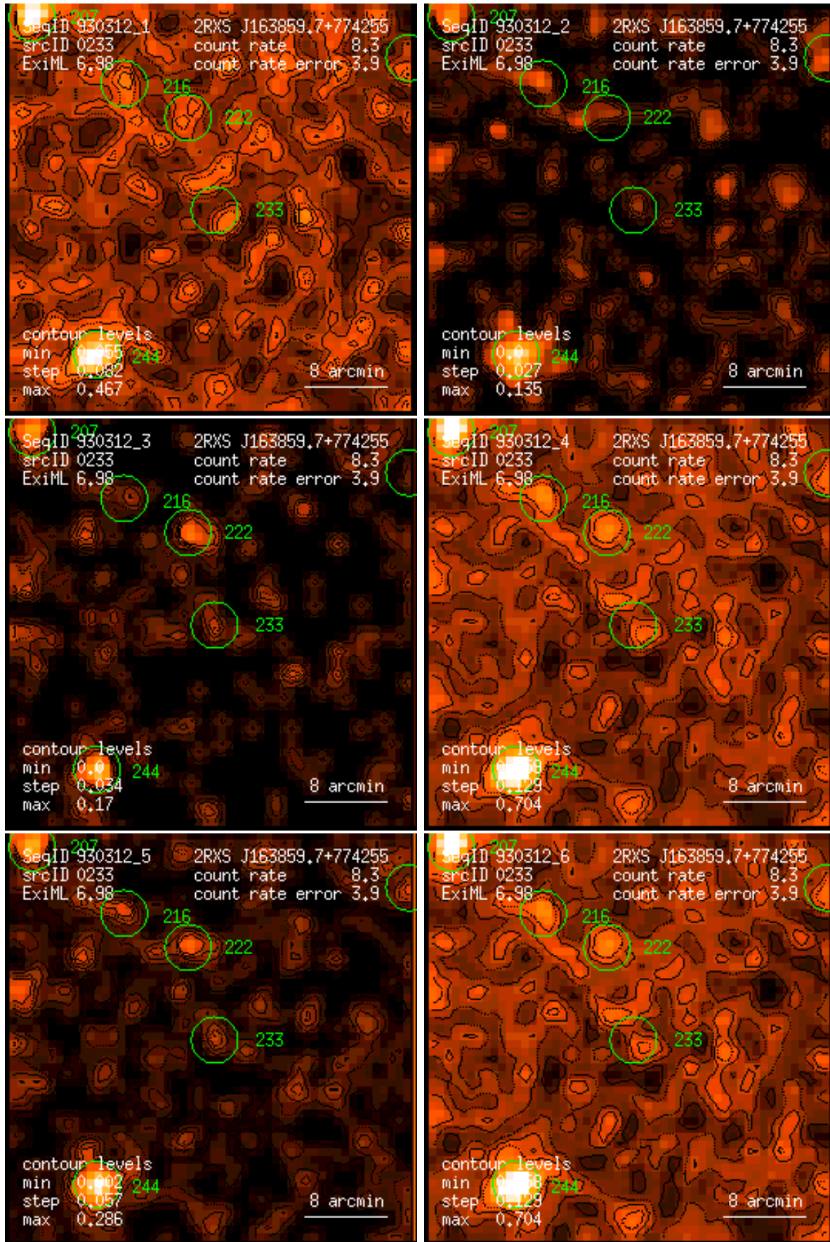
Figure 233: RASS 930312: detection 0233: band rate images, Gaussian filter: (1) PSPC channels 11 – 41, (2) 52 – 90, (3) 91 – 201, (4) 11 – 235, (5) 52 – 201, (6) 11 – 201. Broad band rates in counts/ks. Band rate contour levels in counts/ks/arcmin 2 .
