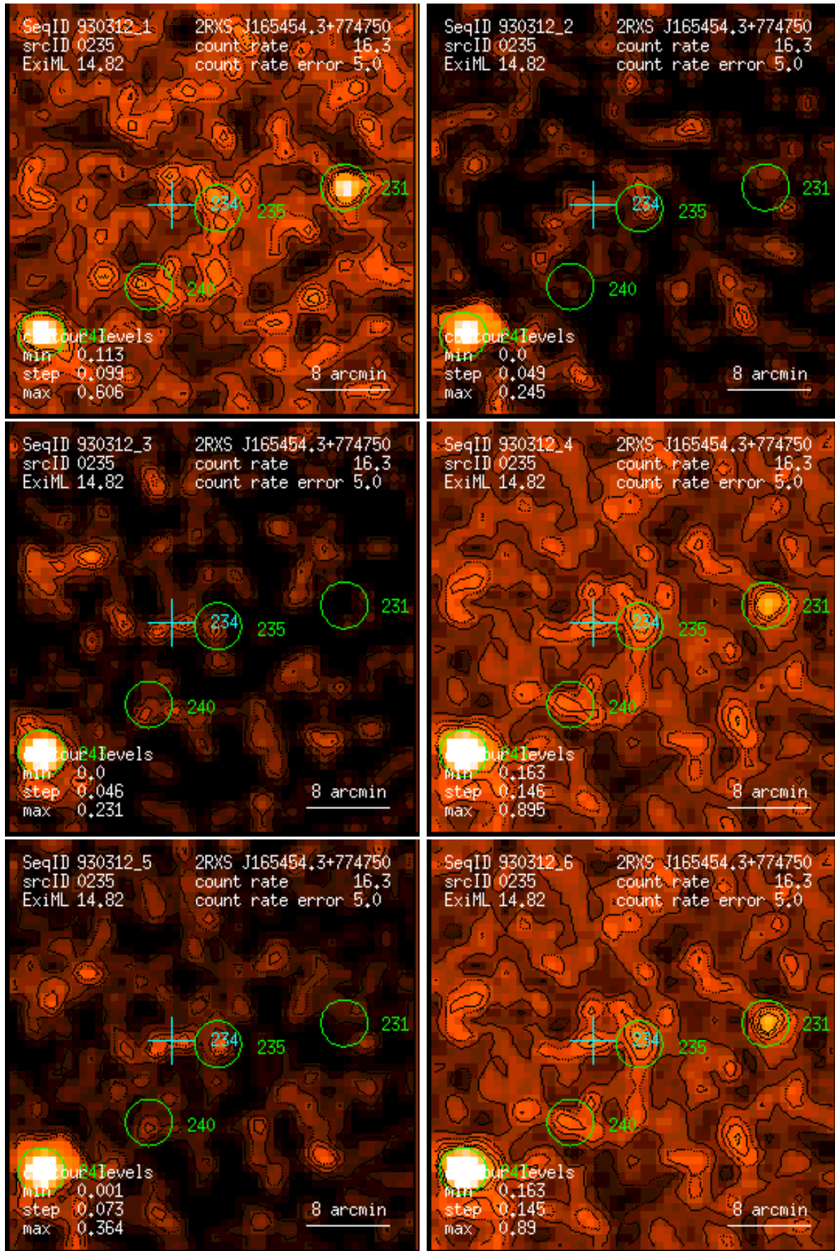
Figure 235: RASS 930312: detection 0235: band rate images, Gaussian filter: (1) PSPC channels 11 – 41, (2) 52 – 90, (3) 91 – 201, (4) 11 – 235, (5) 52 – 201, (6) 11 – 201. Broad band rates in counts/ks. Band rate contour levels in counts/ks/arcmin 2 .
