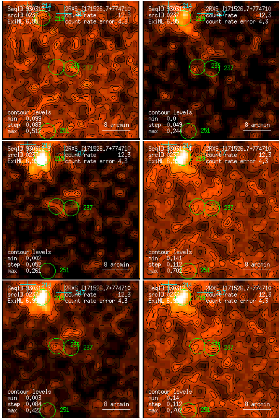
Figure 237: RASS 930312: detection 0237: band rate images, Gaussian filter: (1) PSPC channels 11 – 41, (2) 52 – 90, (3) 91 – 201, (4) 11 – 235, (5) 52 – 201, (6) 11 – 201. Broad band rates in counts/ks. Band rate contour levels in counts/ks/arcmin 2 .
