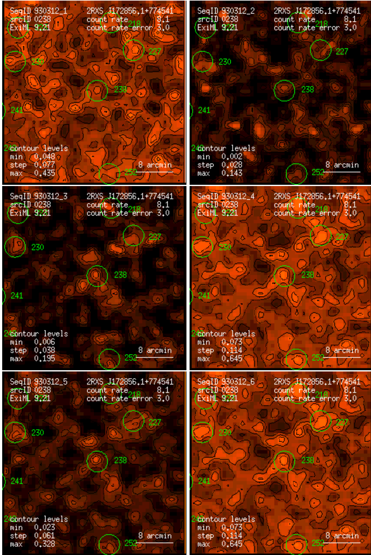
Figure 238: RASS 930312: detection 0238: band rate images, Gaussian filter: (1) PSPC channels 11 – 41, (2) 52 – 90, (3) 91 – 201, (4) 11 – 235, (5) 52 – 201, (6) 11 – 201. Broad band rates in counts/ks. Band rate contour levels in counts/ks/arcmin 2 .
