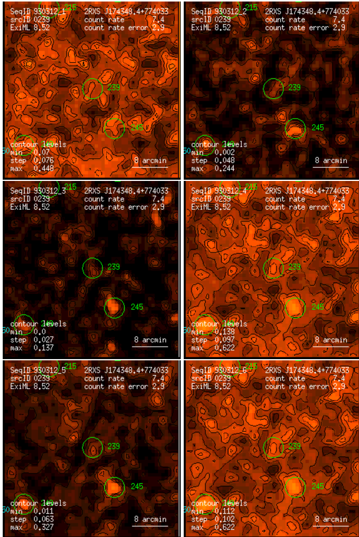
Figure 239: RASS 930312: detection 0239: band rate images, Gaussian filter: (1) PSPC channels 11 – 41, (2) 52 – 90, (3) 91 – 201, (4) 11 – 235, (5) 52 – 201, (6) 11 – 201. Broad band rates in counts/ks. Band rate contour levels in counts/ks/arcmin 2 .
