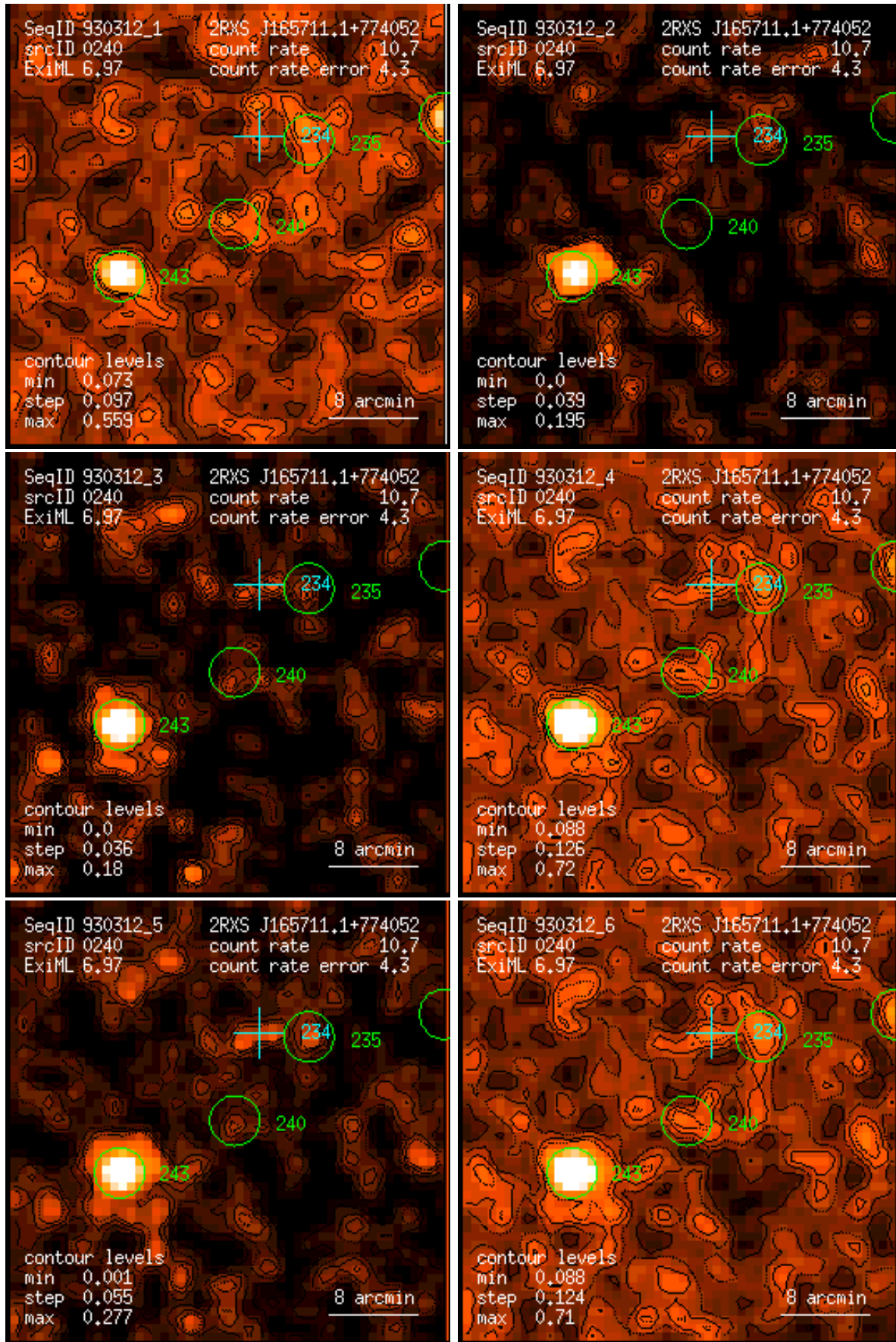
Figure 240: RASS 930312: detection 0240: band rate images, Gaussian filter: (1) PSPC channels 11 – 41, (2) 52 – 90, (3) 91 – 201, (4) 11 – 235, (5) 52 – 201, (6) 11 – 201. Broad band rates in counts/ks. Band rate contour levels in counts/ks/arcmin 2 .
