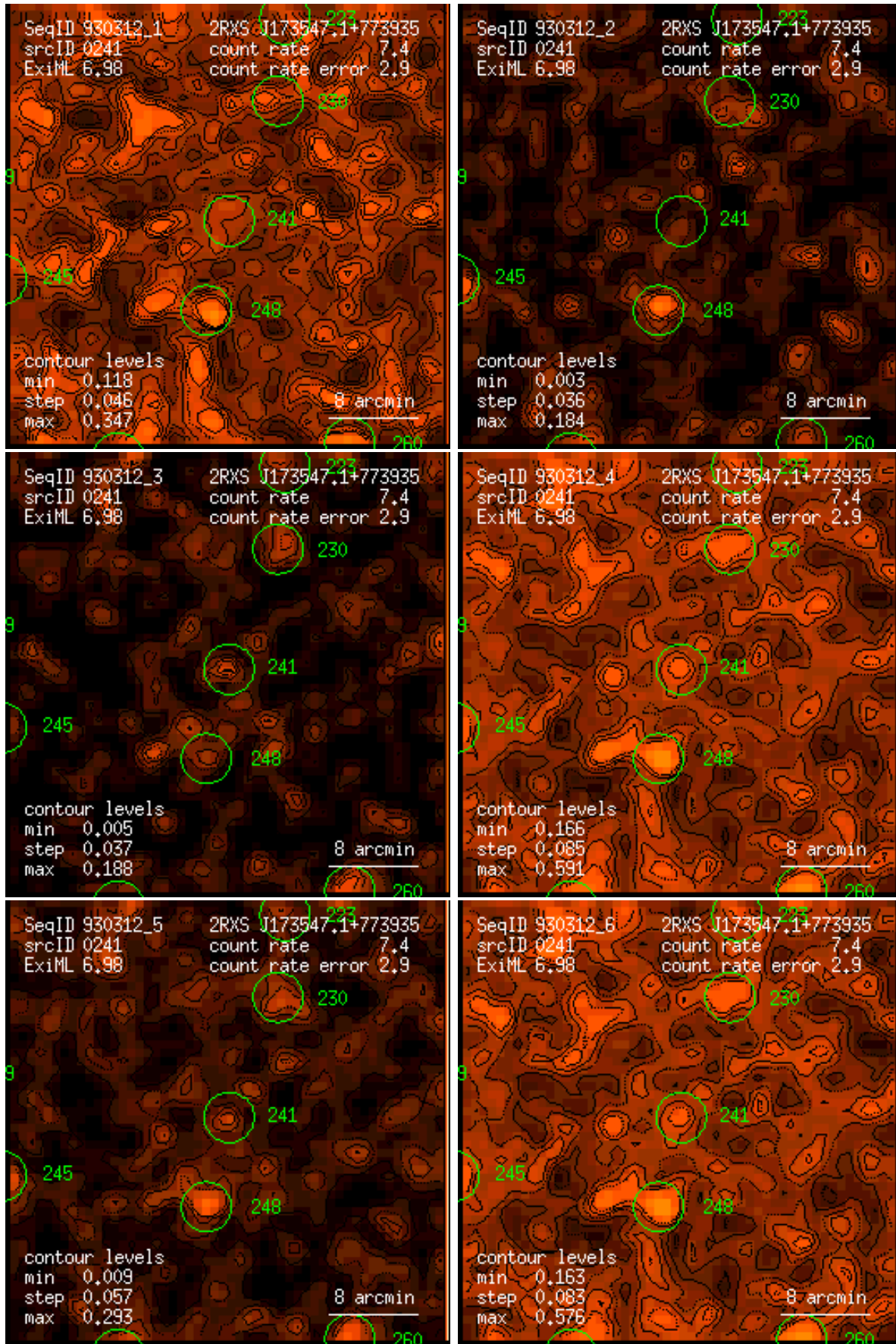
Figure 241: RASS 930312: detection 0241: band rate images, Gaussian filter: (1) PSPC channels 11 – 41, (2) 52 – 90, (3) 91 – 201, (4) 11 – 235, (5) 52 – 201, (6) 11 – 201. Broad band rates in counts/ks. Band rate contour levels in counts/ks/arcmin 2 .
