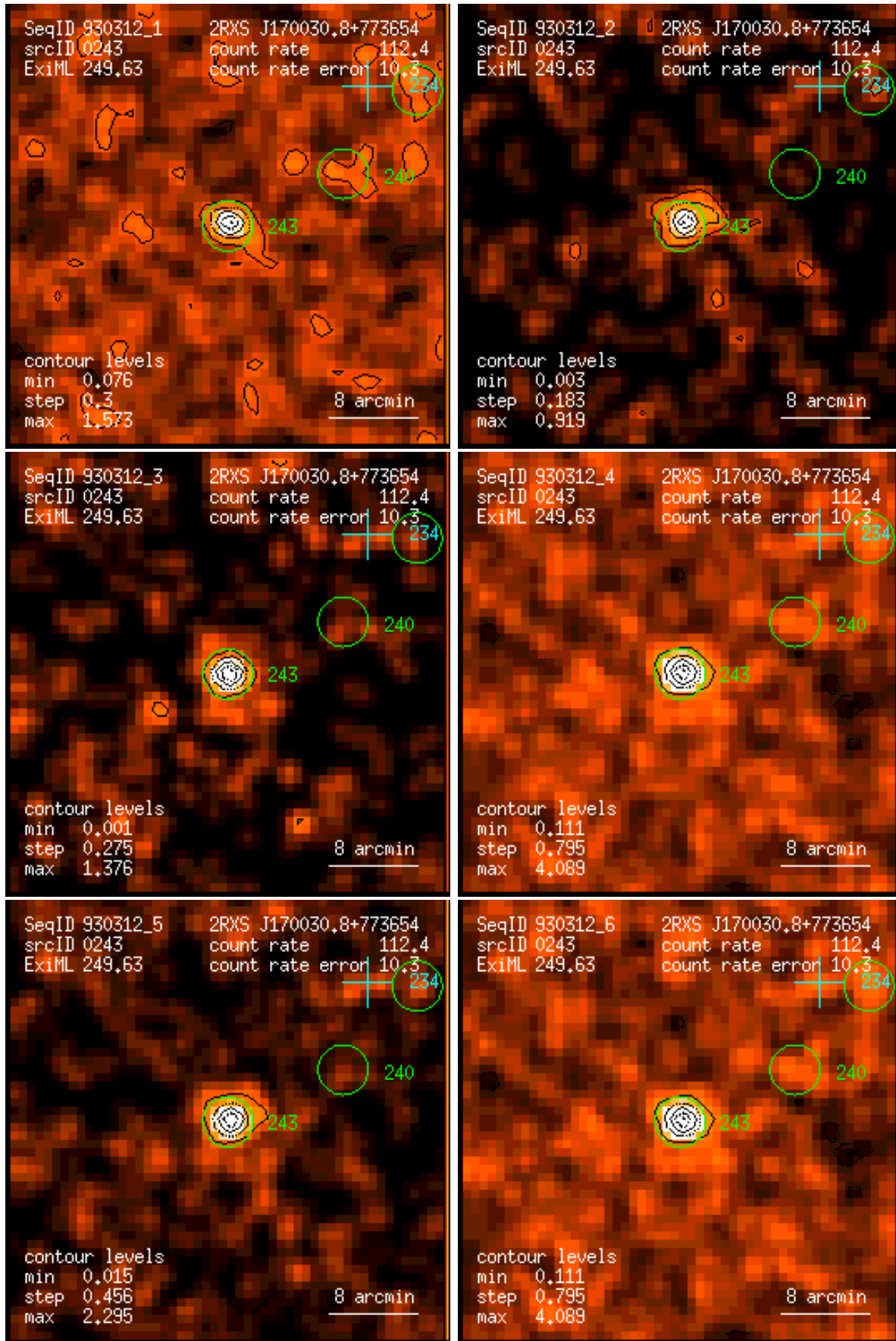
Figure 243: RASS 930312: detection 0243: band rate images, Gaussian filter: (1) PSPC channels 11 – 41, (2) 52 – 90, (3) 91 – 201, (4) 11 – 235, (5) 52 – 201, (6) 11 – 201. Broad band rates in counts/ks. Band rate contour levels in counts/ks/arcmin 2 .
