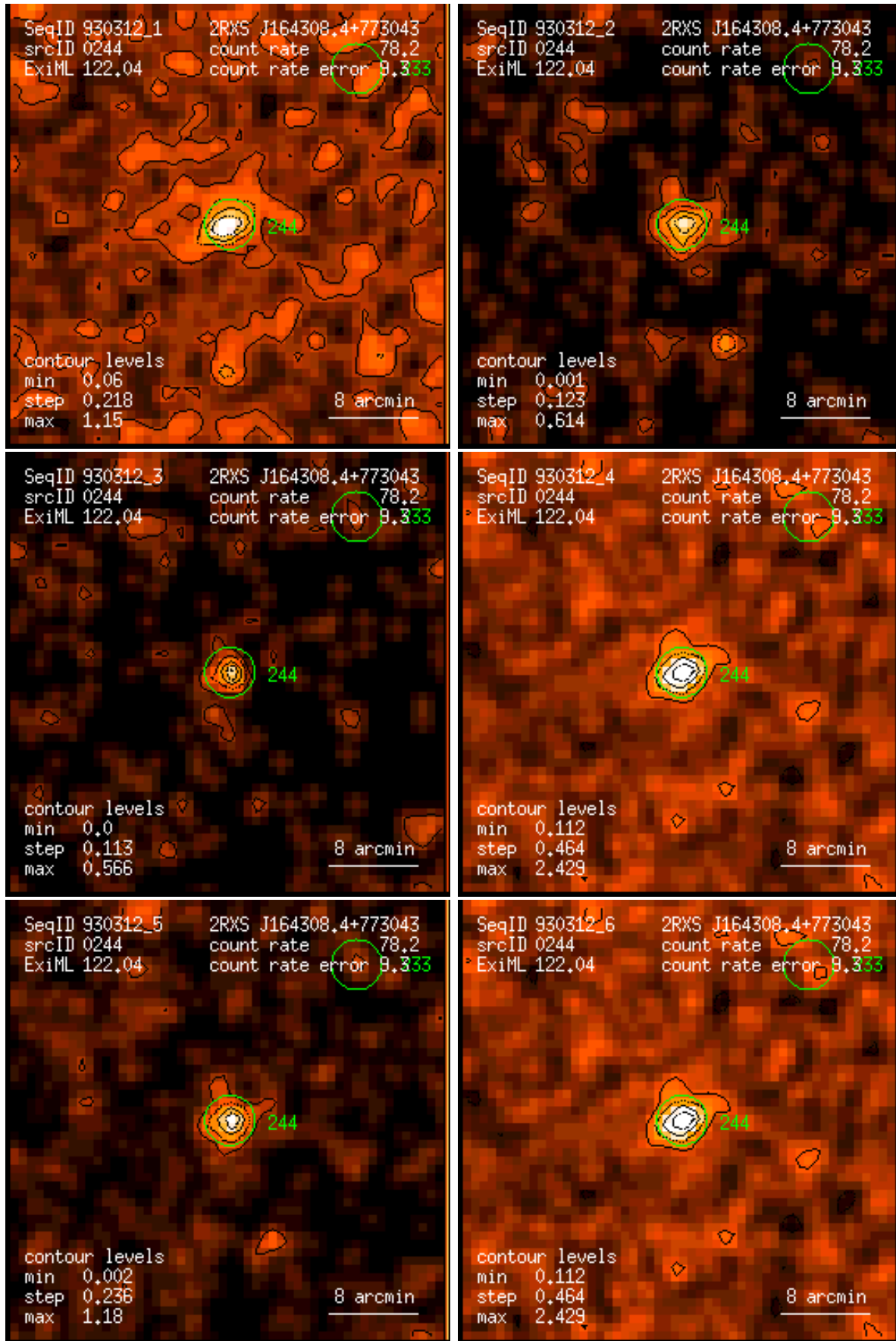
Figure 244: RASS 930312: detection 0244: band rate images, Gaussian filter: (1) PSPC channels 11 – 41, (2) 52 – 90, (3) 91 – 201, (4) 11 – 235, (5) 52 – 201, (6) 11 – 201. Broad band rates in counts/ks. Band rate contour levels in counts/ks/arcmin 2 .
