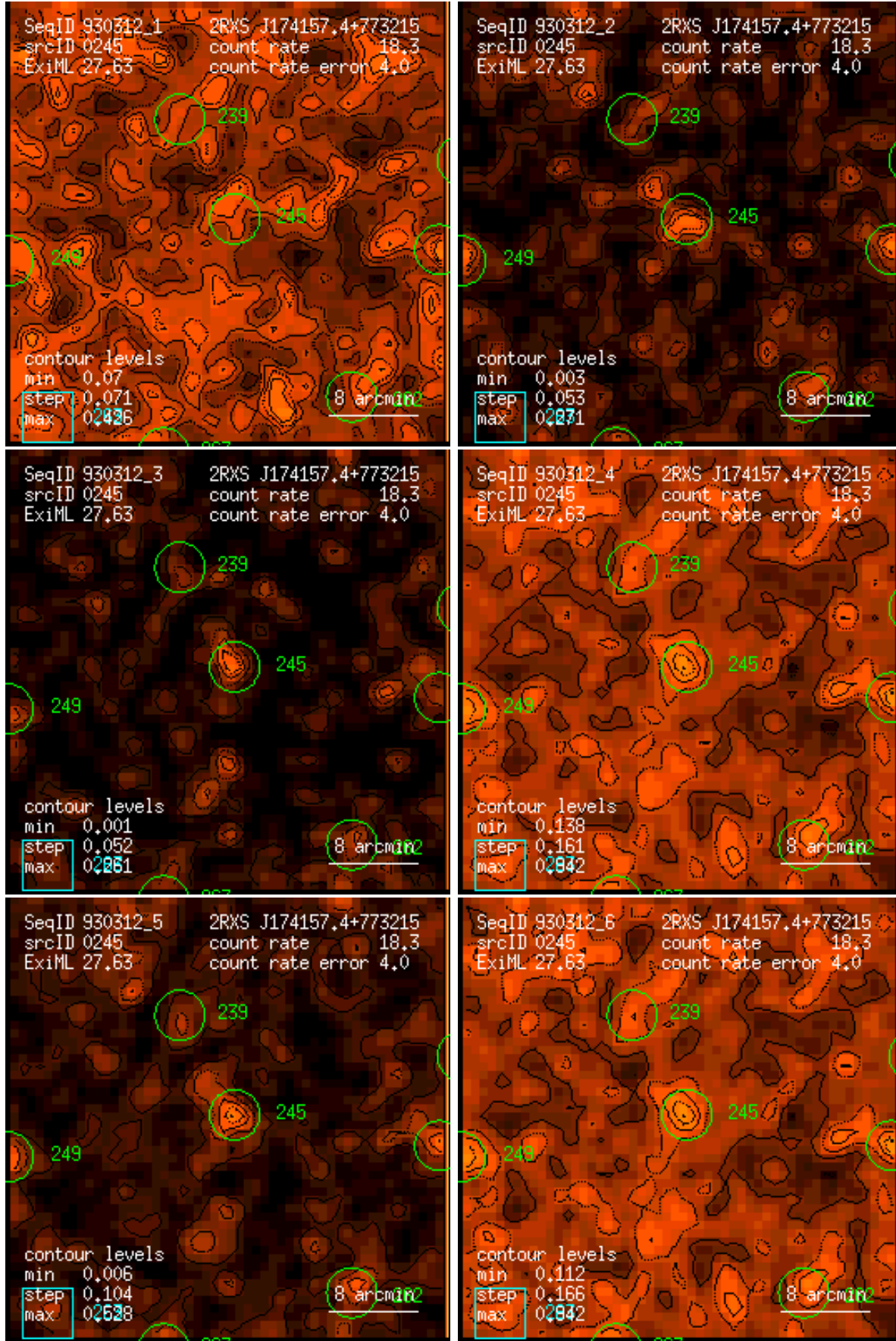
Figure 245: RASS 930312: detection 0245: band rate images, Gaussian filter: (1) PSPC channels 11 – 41, (2) 52 – 90, (3) 91 – 201, (4) 11 – 235, (5) 52 – 201, (6) 11 – 201. Broad band rates in counts/ks. Band rate contour levels in counts/ks/arcmin 2 .
