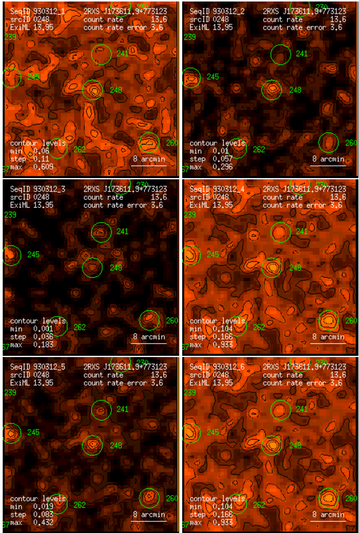
Figure 248: RASS 930312: detection 0248: band rate images, Gaussian filter: (1) PSPC channels 11 – 41, (2) 52 – 90, (3) 91 – 201, (4) 11 – 235, (5) 52 – 201, (6) 11 – 201. Broad band rates in counts/ks. Band rate contour levels in counts/ks/arcmin 2 .
