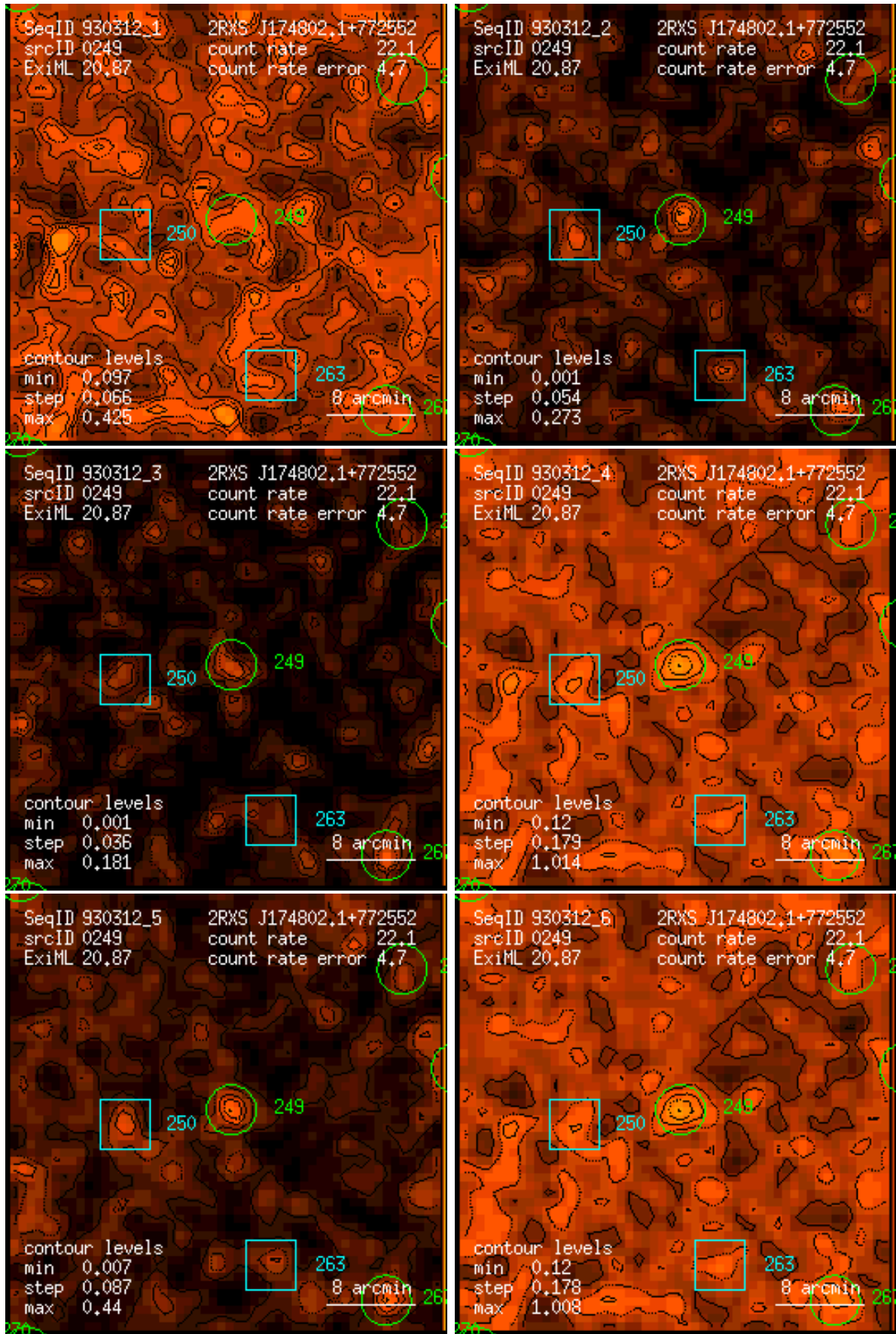
Figure 249: RASS 930312: detection 0249: band rate images, Gaussian filter: (1) PSPC channels 11 – 41, (2) 52 – 90, (3) 91 – 201, (4) 11 – 235, (5) 52 – 201, (6) 11 – 201. Broad band rates in counts/ks. Band rate contour levels in counts/ks/arcmin 2 .
