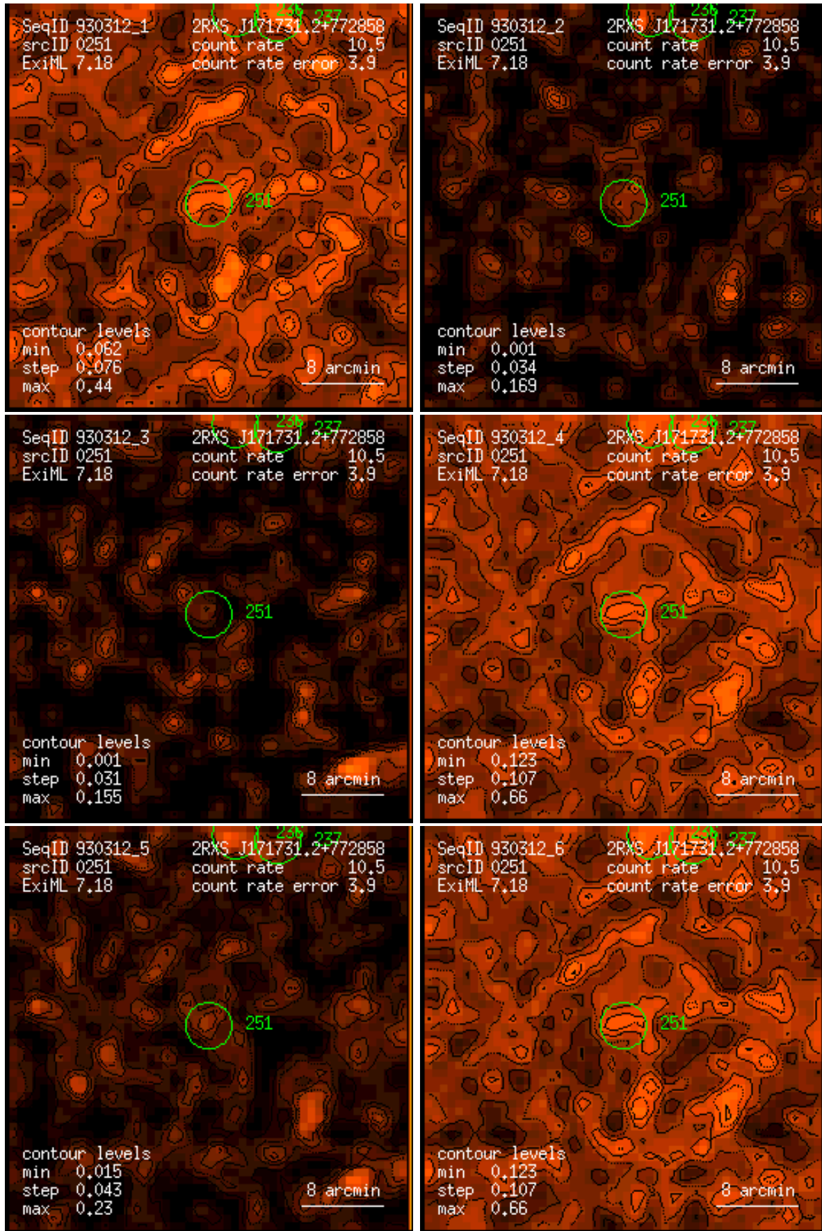
Figure 251: RASS 930312: detection 0251: band rate images, Gaussian filter: (1) PSPC channels 11 – 41, (2) 52 – 90, (3) 91 – 201, (4) 11 – 235, (5) 52 – 201, (6) 11 – 201. Broad band rates in counts/ks. Band rate contour levels in counts/ks/arcmin 2 .
