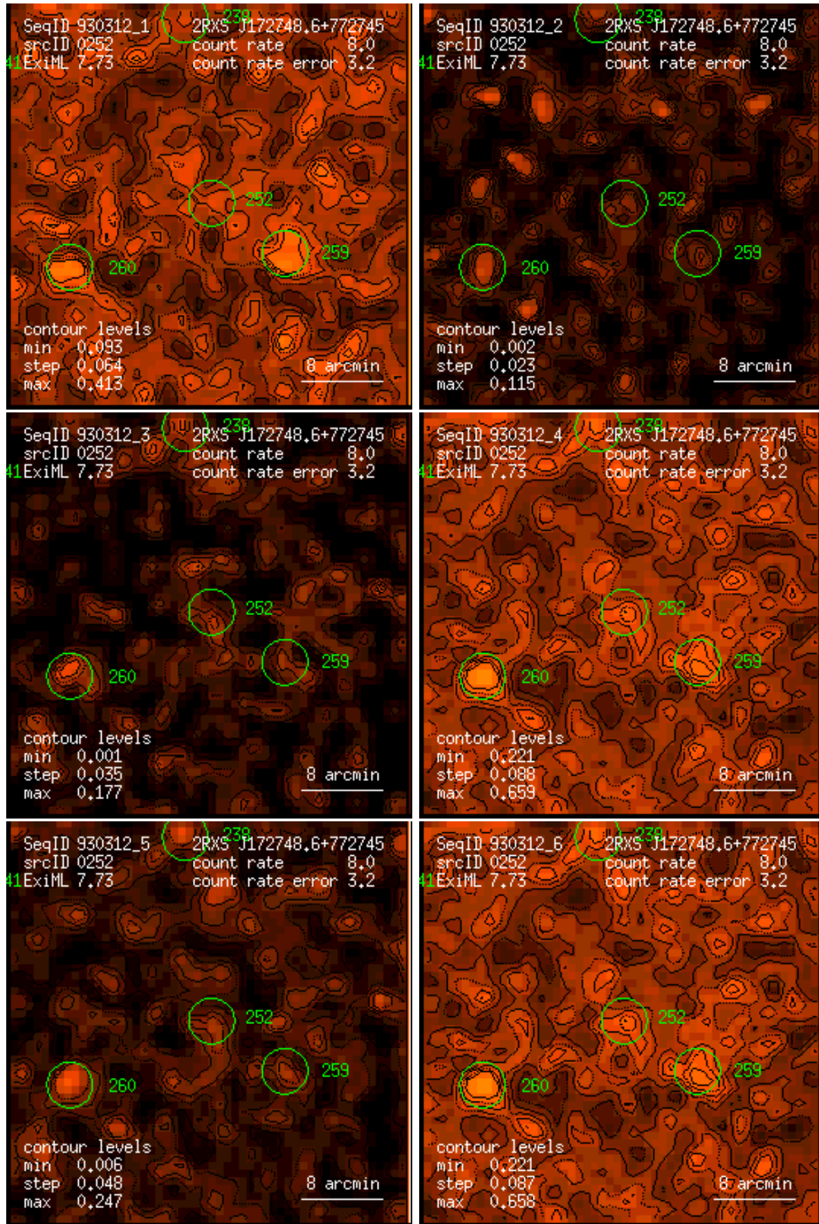
Figure 252: RASS 930312: detection 0252: band rate images, Gaussian filter: (1) PSPC channels 11 – 41, (2) 52 – 90, (3) 91 – 201, (4) 11 – 235, (5) 52 – 201, (6) 11 – 201. Broad band rates in counts/ks. Band rate contour levels in counts/ks/arcmin 2 .
