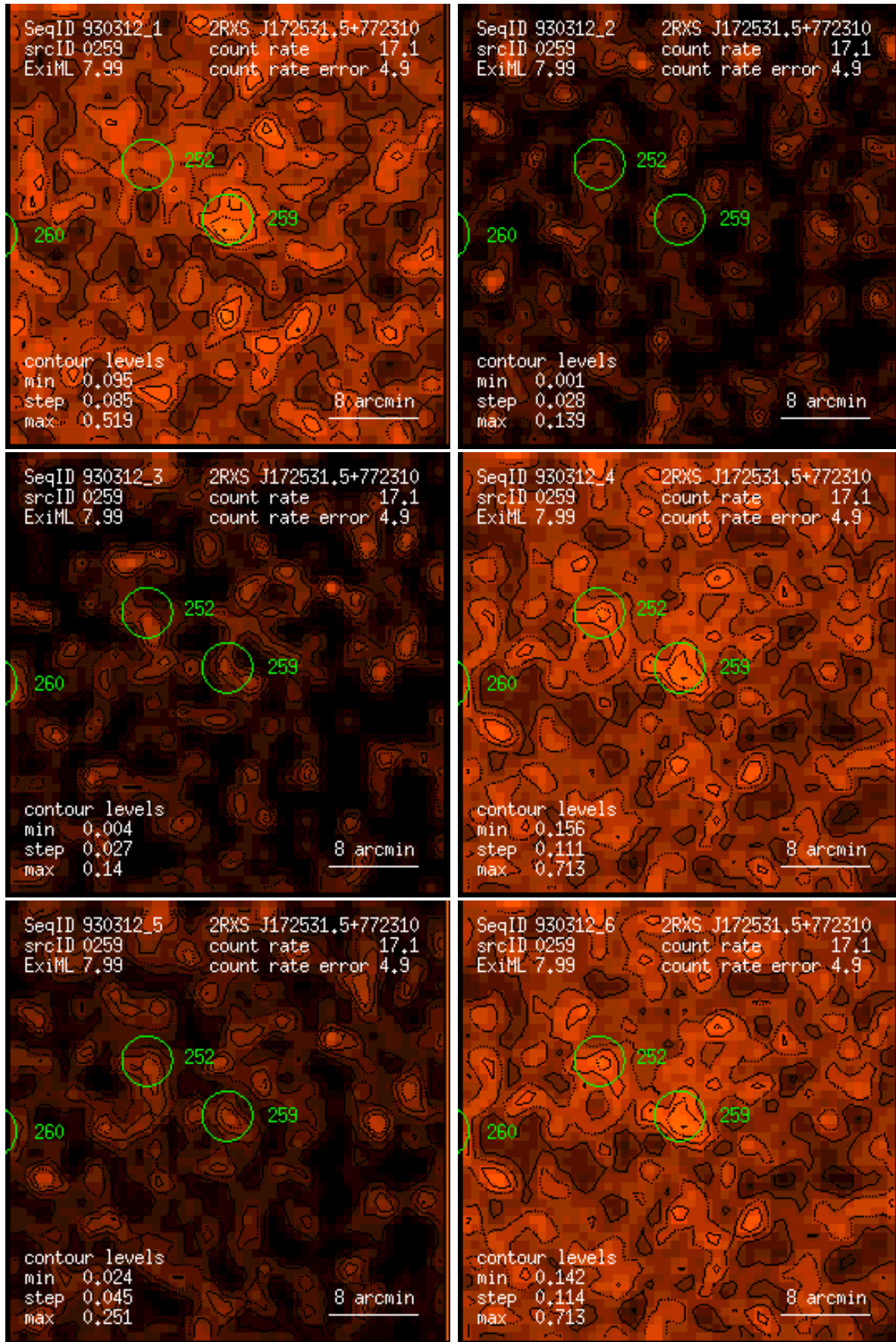
Figure 259: RASS 930312: detection 0259: band rate images, Gaussian filter: (1) PSPC channels 11 – 41, (2) 52 – 90, (3) 91 – 201, (4) 11 – 235, (5) 52 – 201, (6) 11 – 201. Broad band rates in counts/ks. Band rate contour levels in counts/ks/arcmin 2 .
