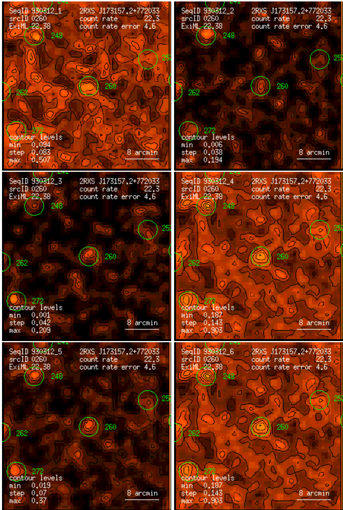
Figure 260: RASS 930312: detection 0260: band rate images, Gaussian filter: (1) PSPC channels 11 – 41, (2) 52 – 90, (3) 91 – 201, (4) 11 – 235, (5) 52 – 201, (6) 11 – 201. Broad band rates in counts/ks. Band rate contour levels in counts/ks/arcmin 2 .
