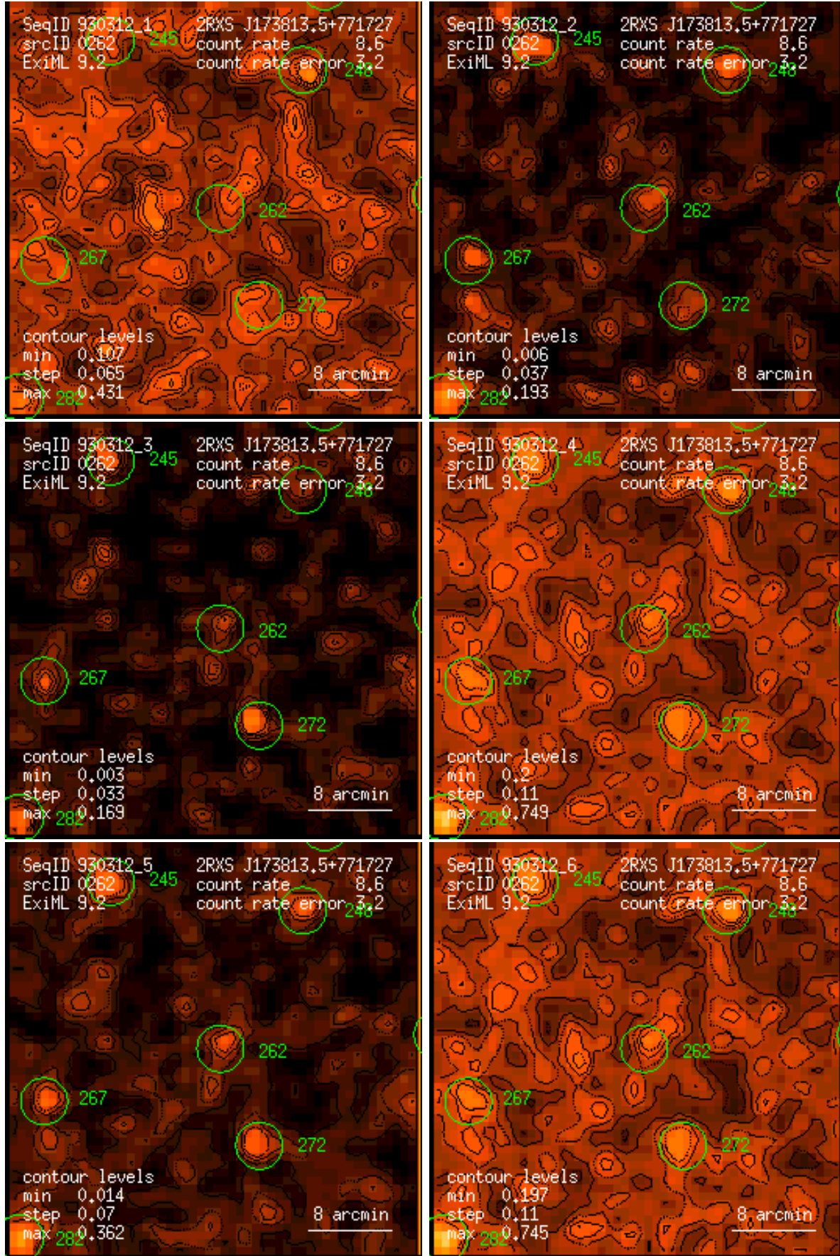
Figure 262: RASS 930312: detection 0262: band rate images, Gaussian filter: (1) PSPC channels 11 – 41, (2) 52 – 90, (3) 91 – 201, (4) 11 – 235, (5) 52 – 201, (6) 11 – 201. Broad band rates in counts/ks. Band rate contour levels in counts/ks/arcmin 2 .
