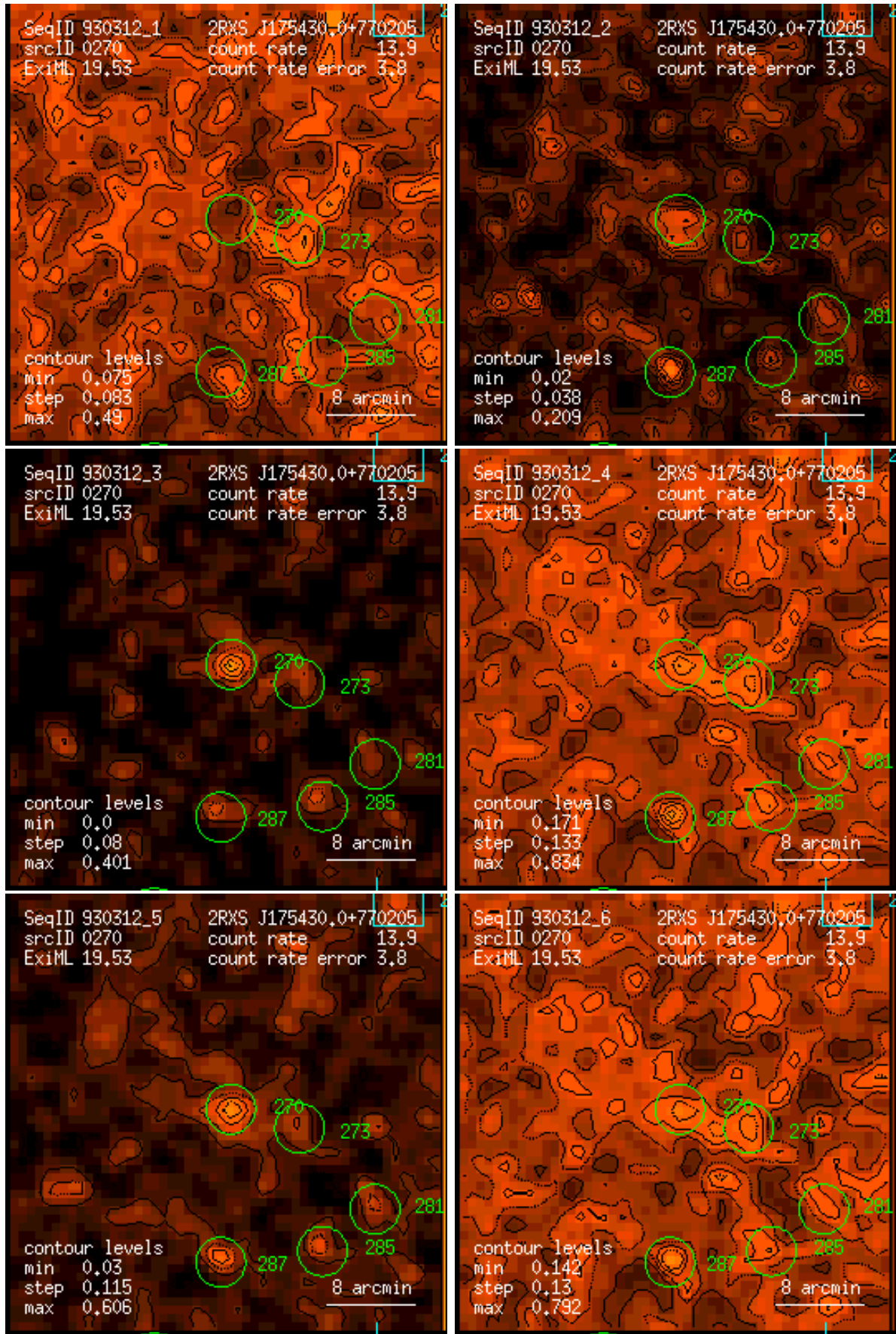
Figure 270: RASS 930312: detection 0270: band rate images, Gaussian filter: (1) PSPC channels 11 – 41, (2) 52 – 90, (3) 91 – 201, (4) 11 – 235, (5) 52 – 201, (6) 11 – 201. Broad band rates in counts/ks. Band rate contour levels in counts/ks/arcmin 2 .
