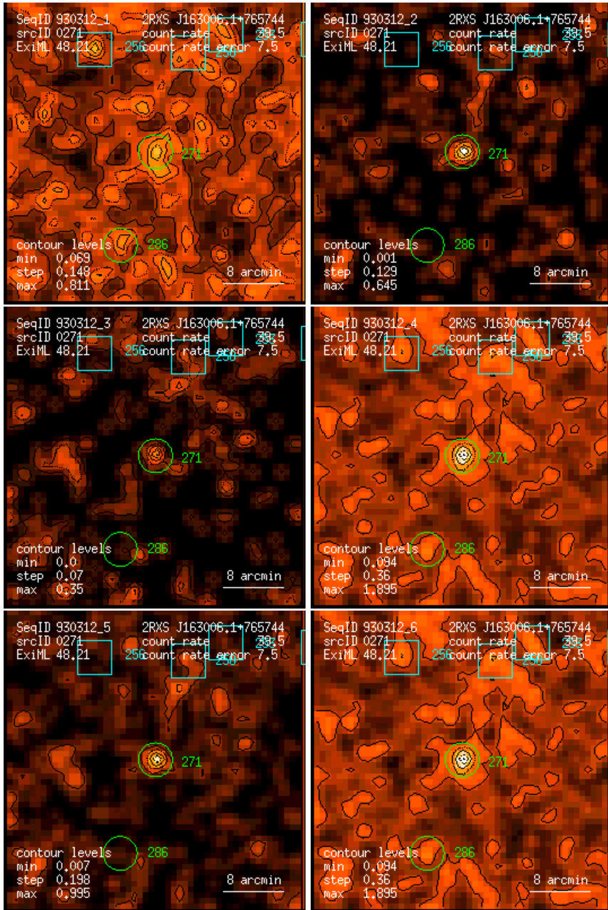
Figure 271: RASS 930312: detection 0271: band rate images, Gaussian filter: (1) PSPC channels 11 – 41, (2) 52 – 90, (3) 91 – 201, (4) 11 – 235, (5) 52 – 201, (6) 11 – 201. Broad band rates in counts/ks. Band rate contour levels in counts/ks/arcmin 2 .
