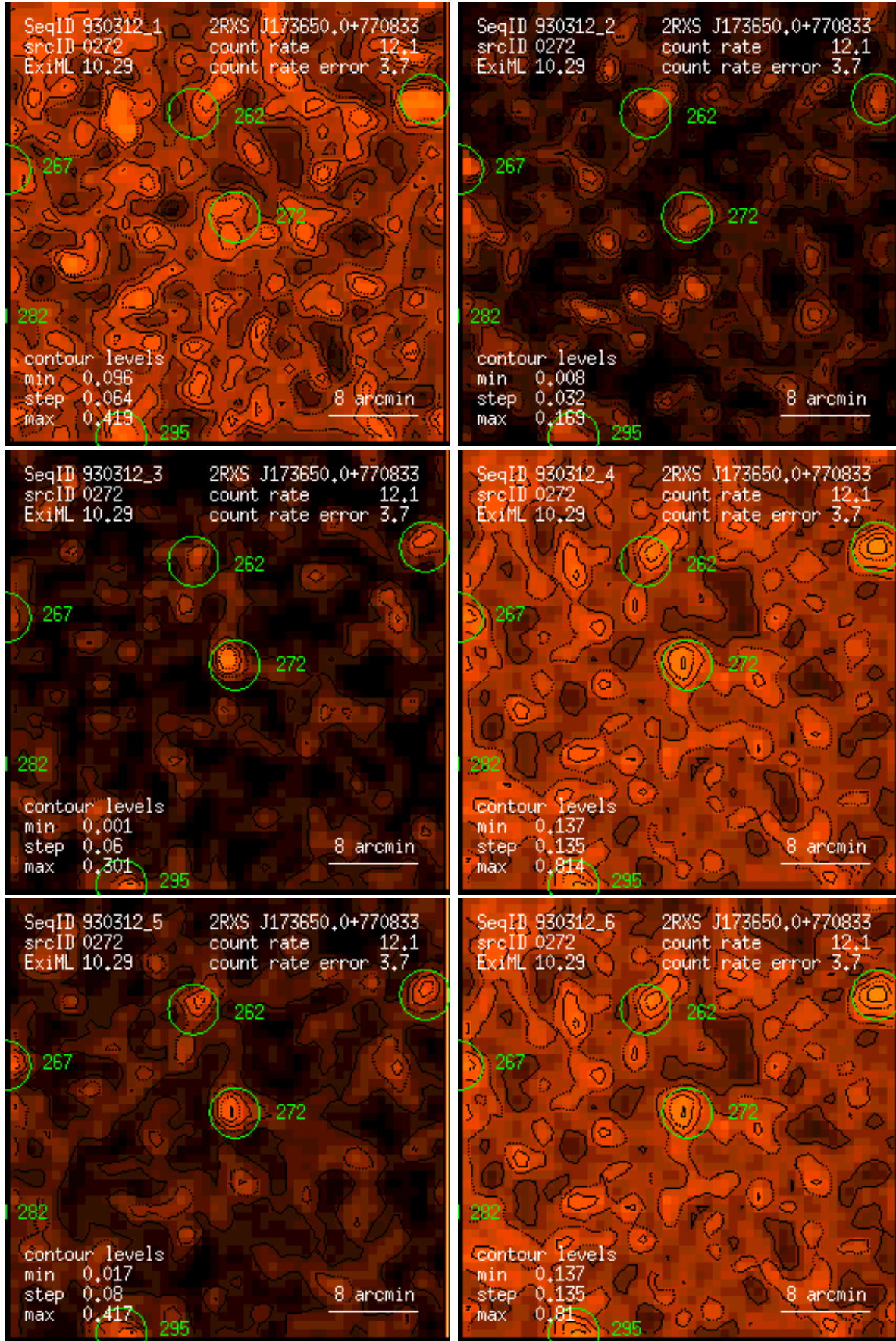
Figure 272: RASS 930312: detection 0272: band rate images, Gaussian filter: (1) PSPC channels 11 – 41, (2) 52 – 90, (3) 91 – 201, (4) 11 – 235, (5) 52 – 201, (6) 11 – 201. Broad band rates in counts/ks. Band rate contour levels in counts/ks/arcmin 2 .
