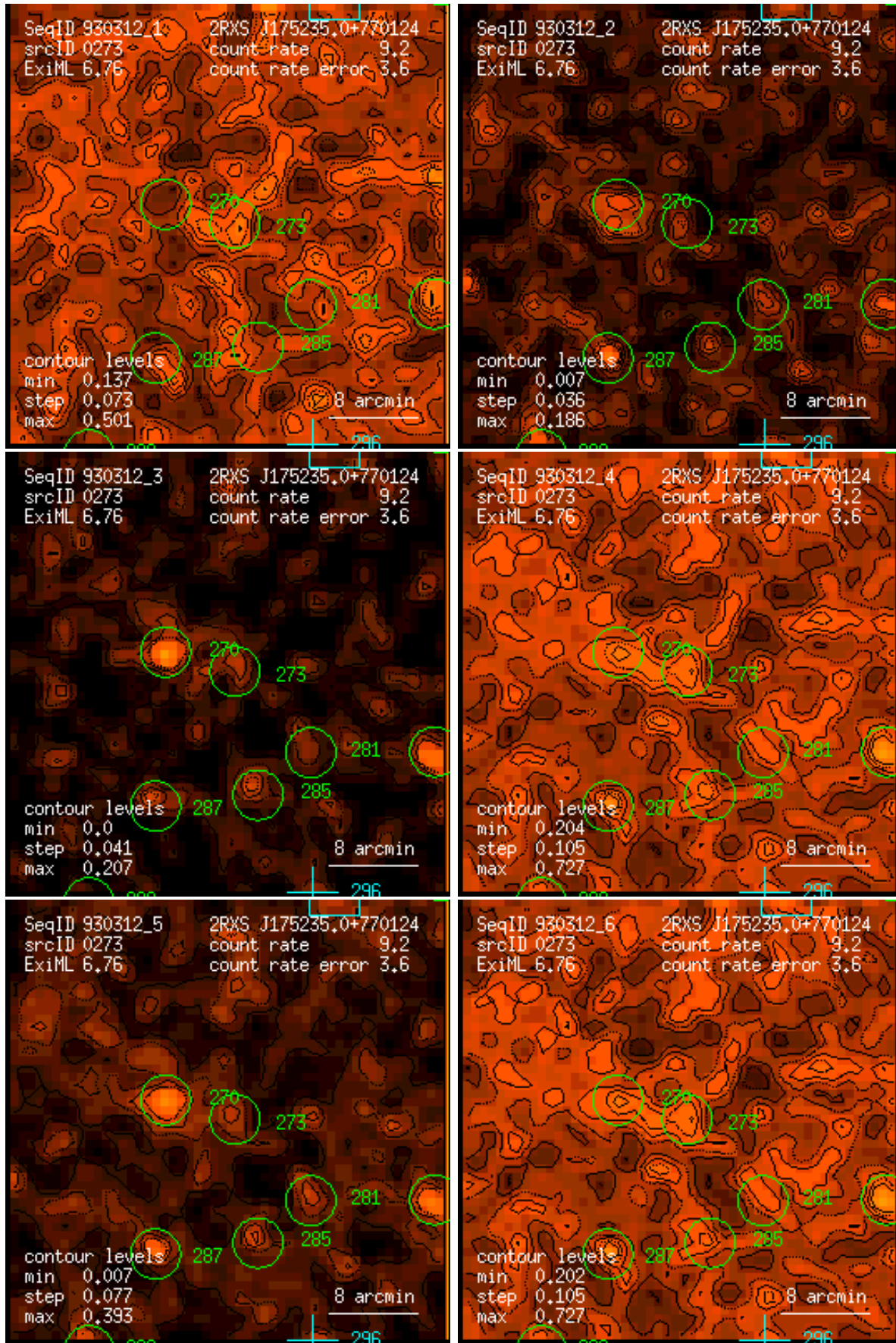
Figure 273: RASS 930312: detection 0273: band rate images, Gaussian filter: (1) PSPC channels 11 – 41, (2) 52 – 90, (3) 91 – 201, (4) 11 – 235, (5) 52 – 201, (6) 11 – 201. Broad band rates in counts/ks. Band rate contour levels in counts/ks/arcmin 2 .
