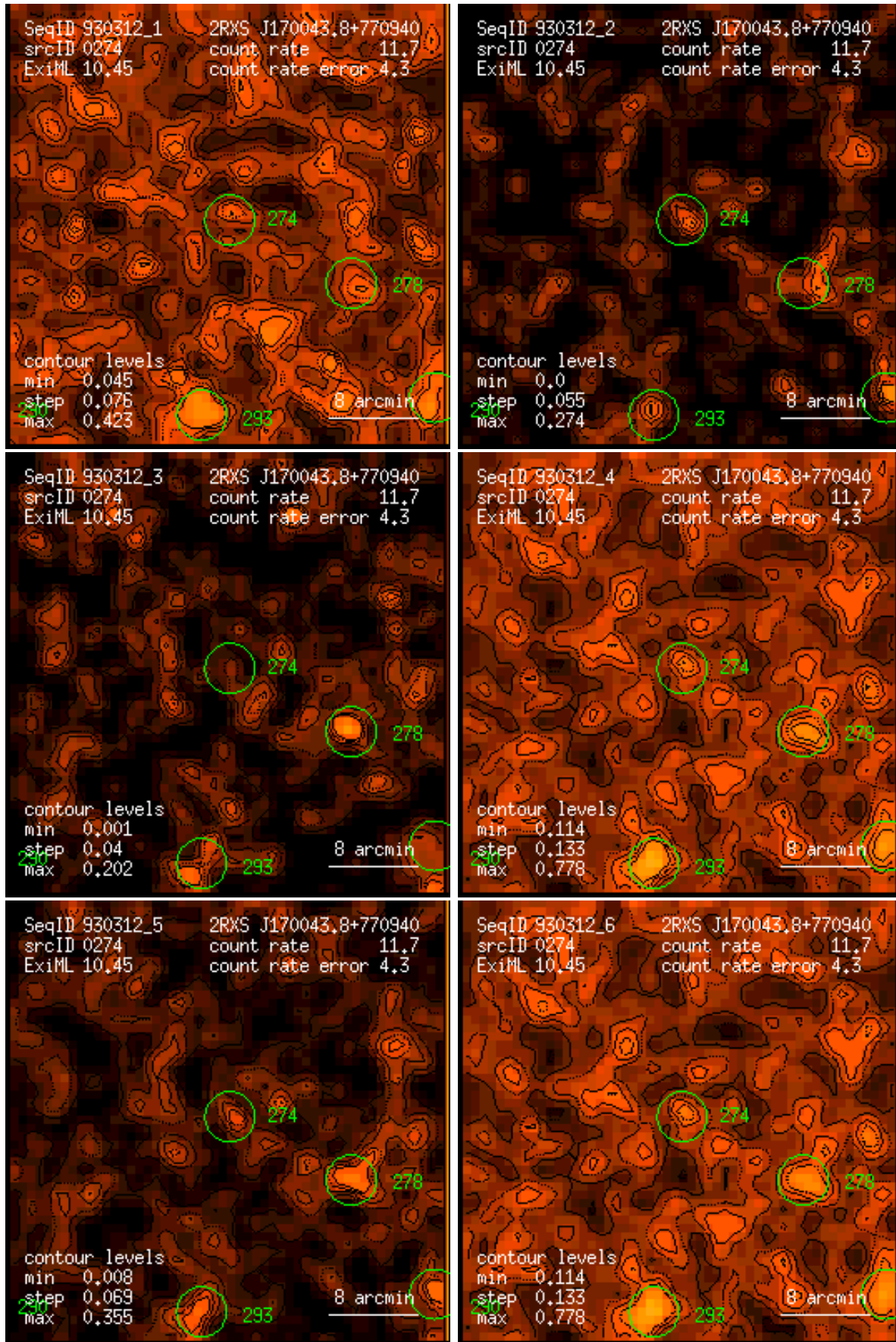
Figure 274: RASS 930312: detection 0274: band rate images, Gaussian filter: (1) PSPC channels 11 – 41, (2) 52 – 90, (3) 91 – 201, (4) 11 – 235, (5) 52 – 201, (6) 11 – 201. Broad band rates in counts/ks. Band rate contour levels in counts/ks/arcmin 2 .
